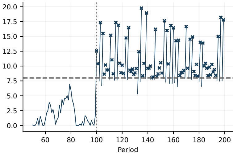
One-sided CUSUM
