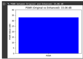
Fig.8 PSNR Result
