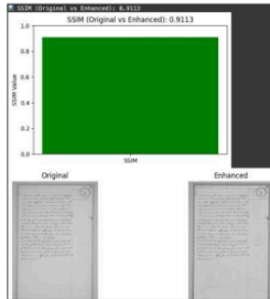
Fig.9 SSIM Result
