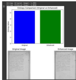
Fig.10 Entropy Result
