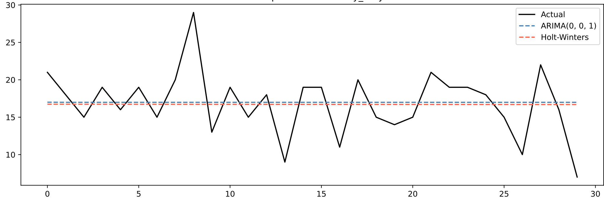
Model Comparison — severity_Very Low
