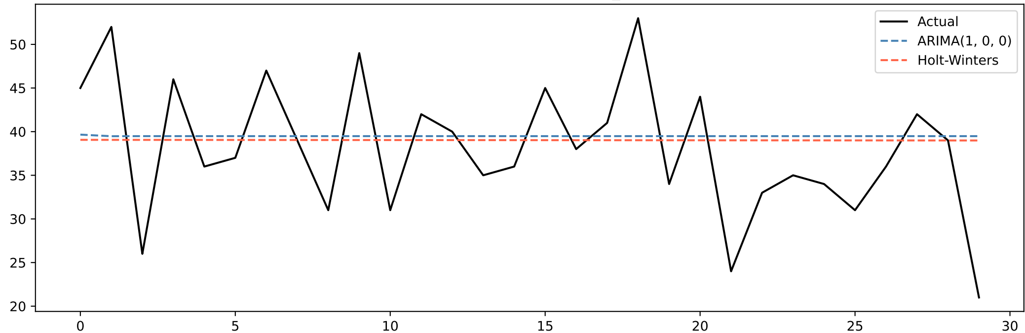
Model Comparison — severity_Medium
