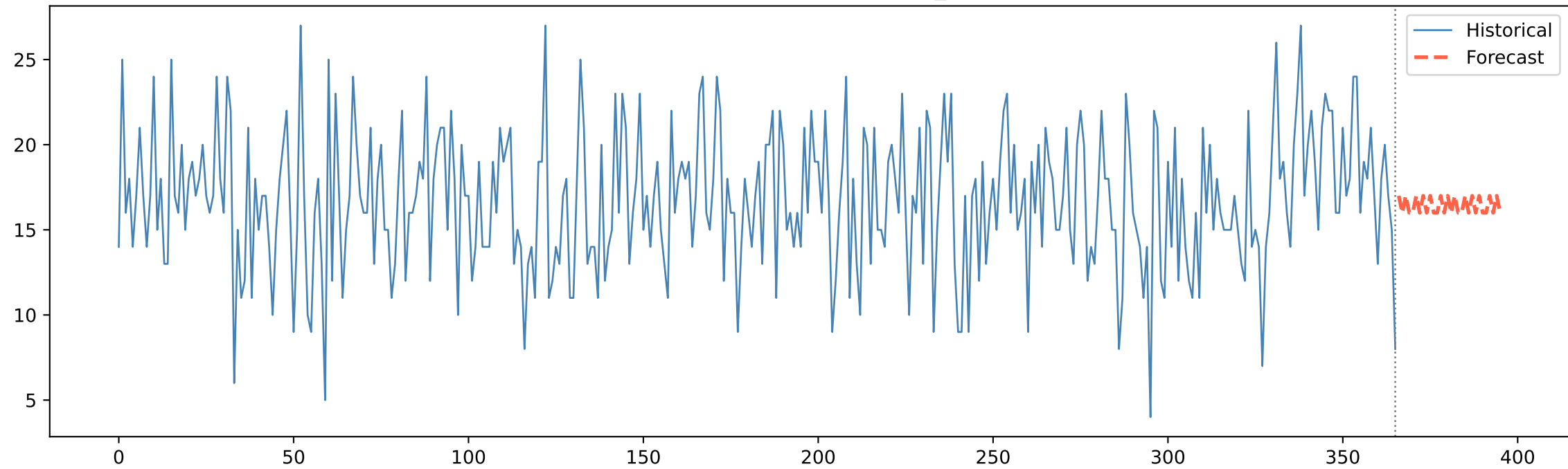
30-Day Forecast — severity_Low
