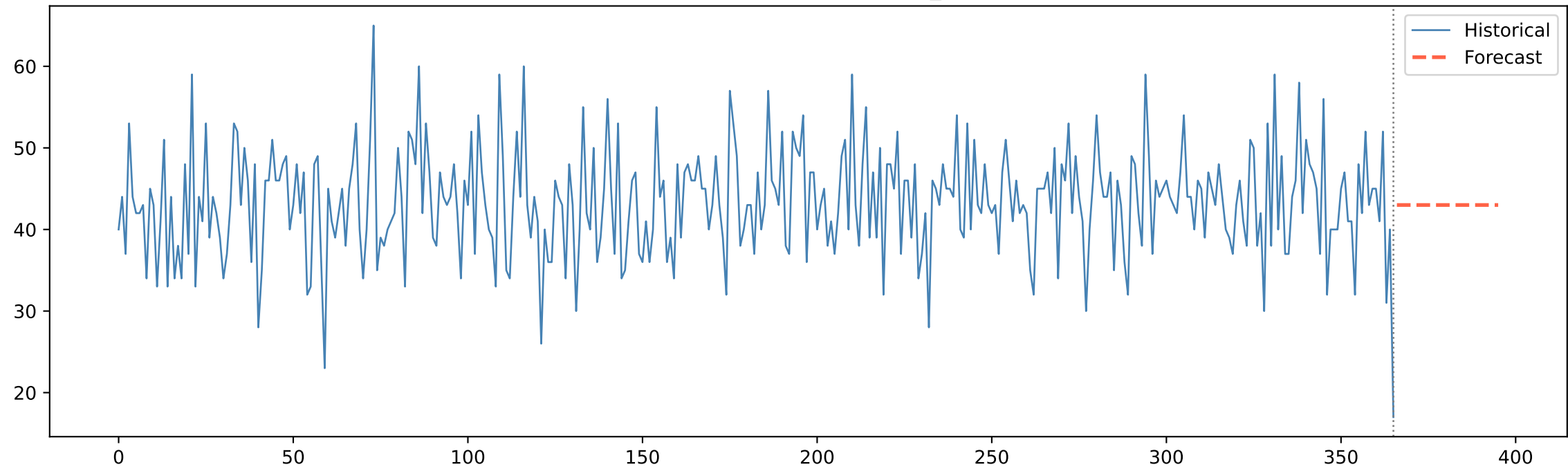
30-Day Forecast — severity_High
