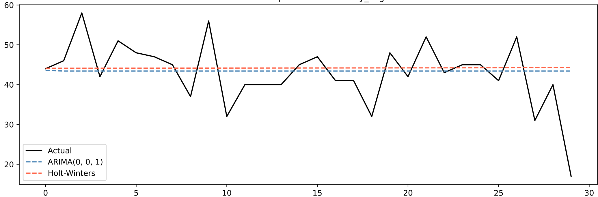
Model Comparison — severity_High
