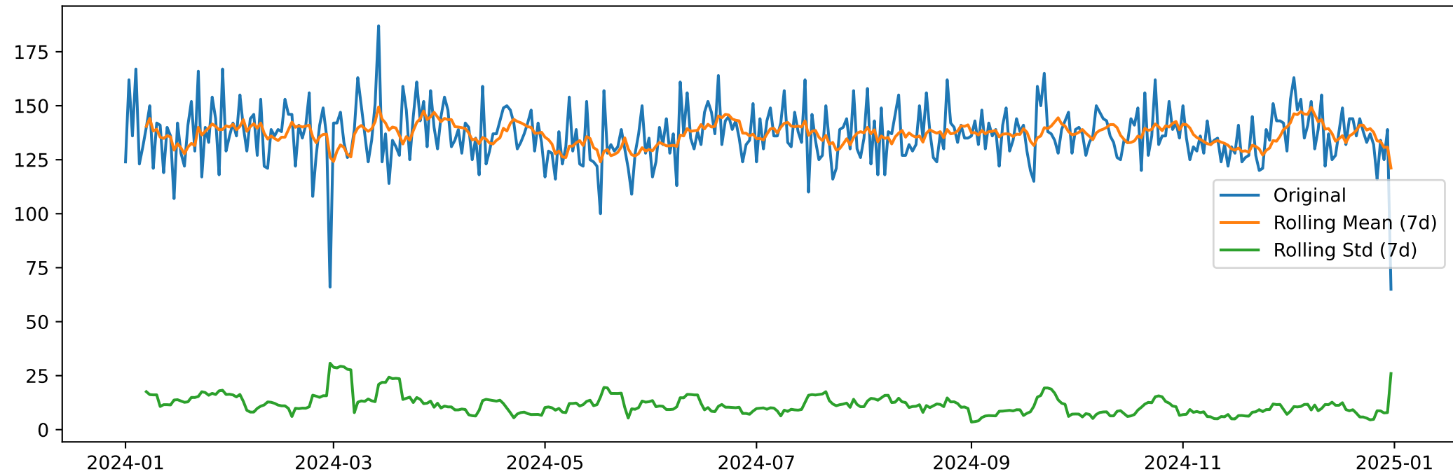
Total Incidents — Rolling Statistics
