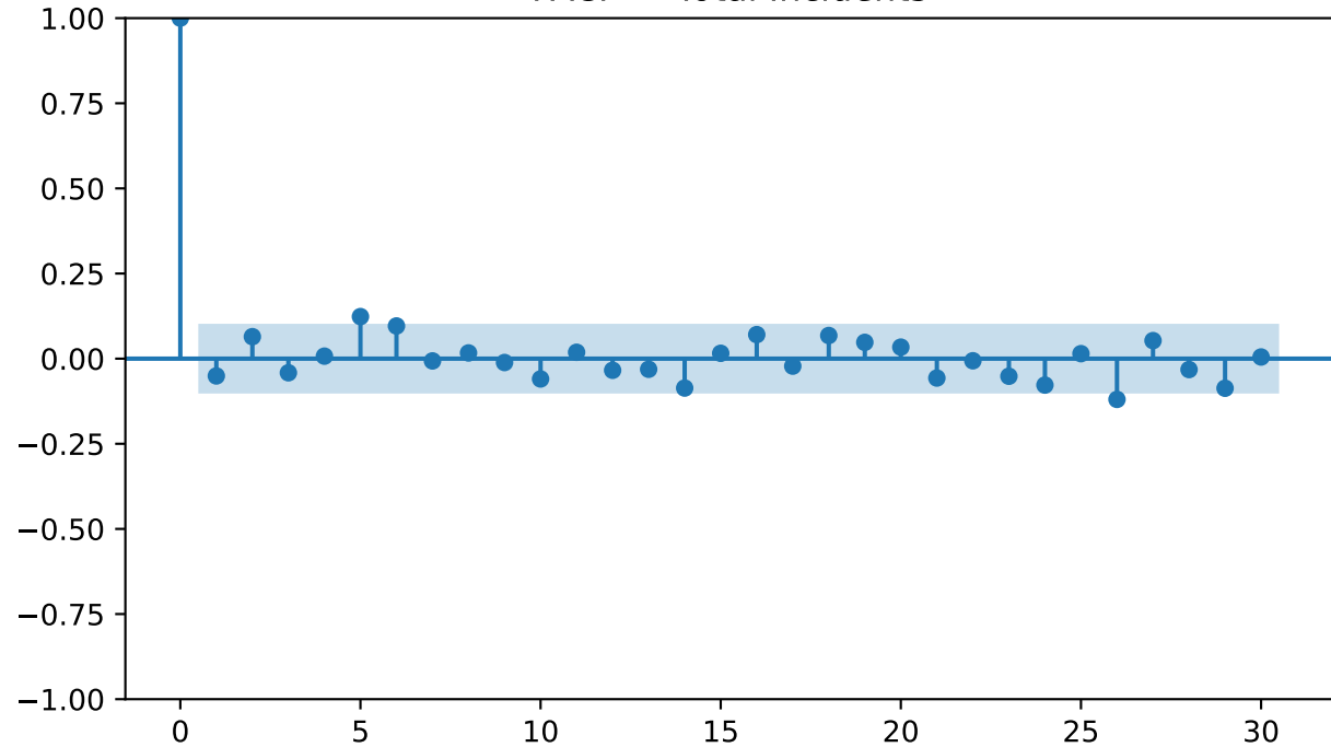
PACF — Total Incidents
