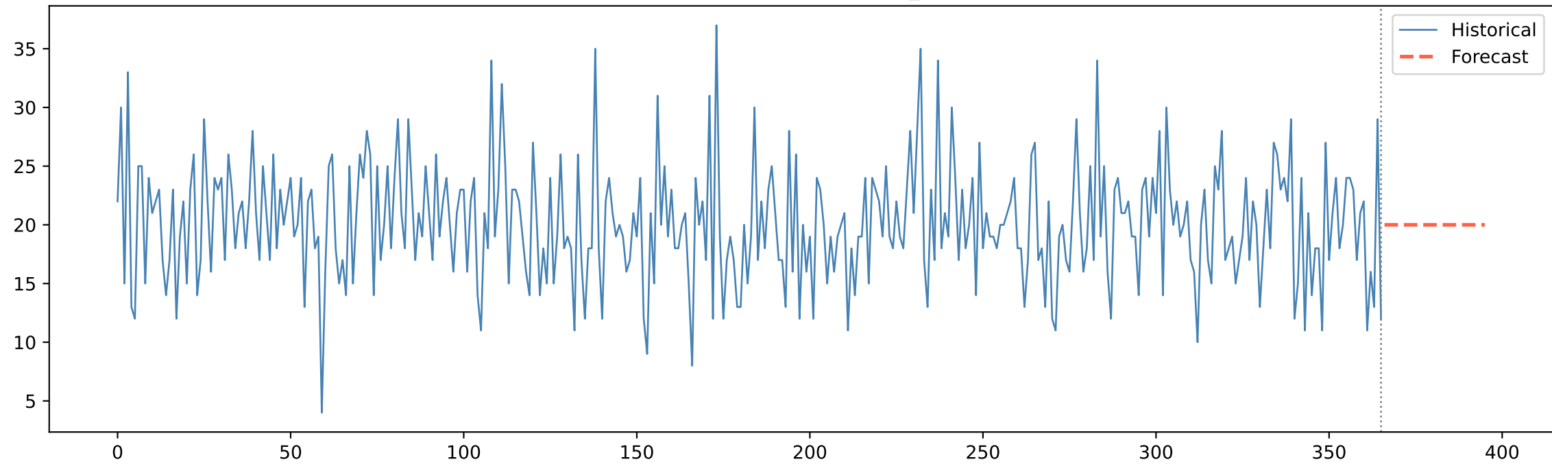
30-Day Forecast — severity_Critical
