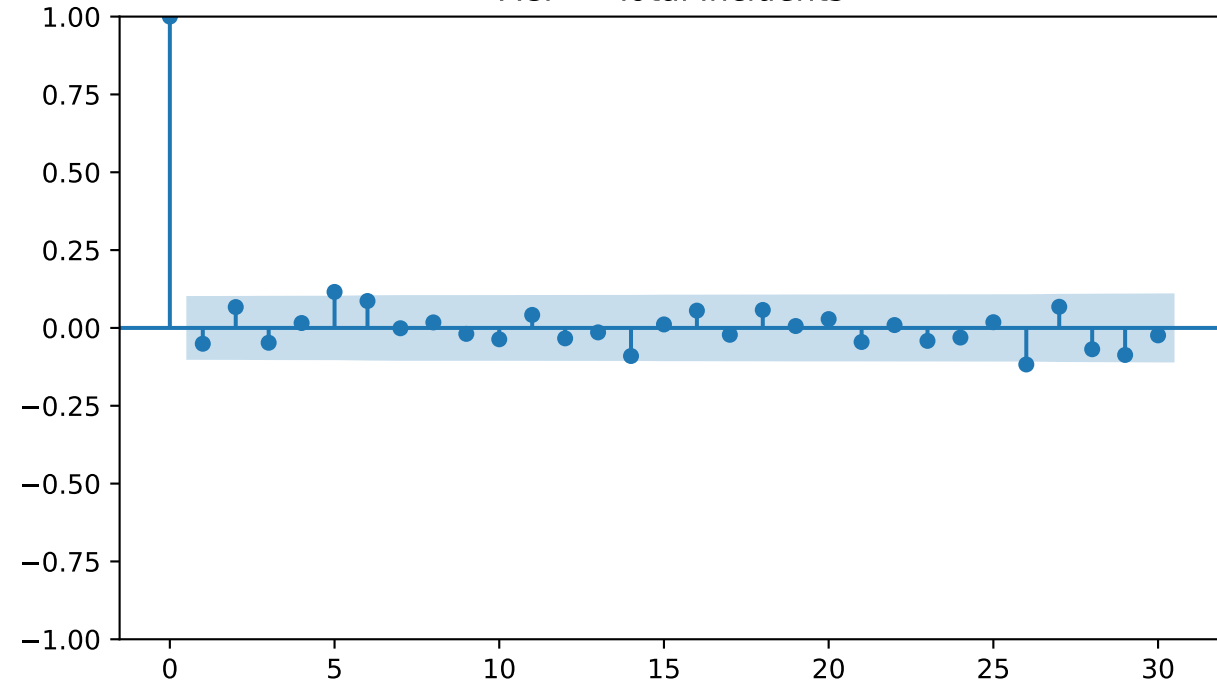
ACF — Total Incidents
