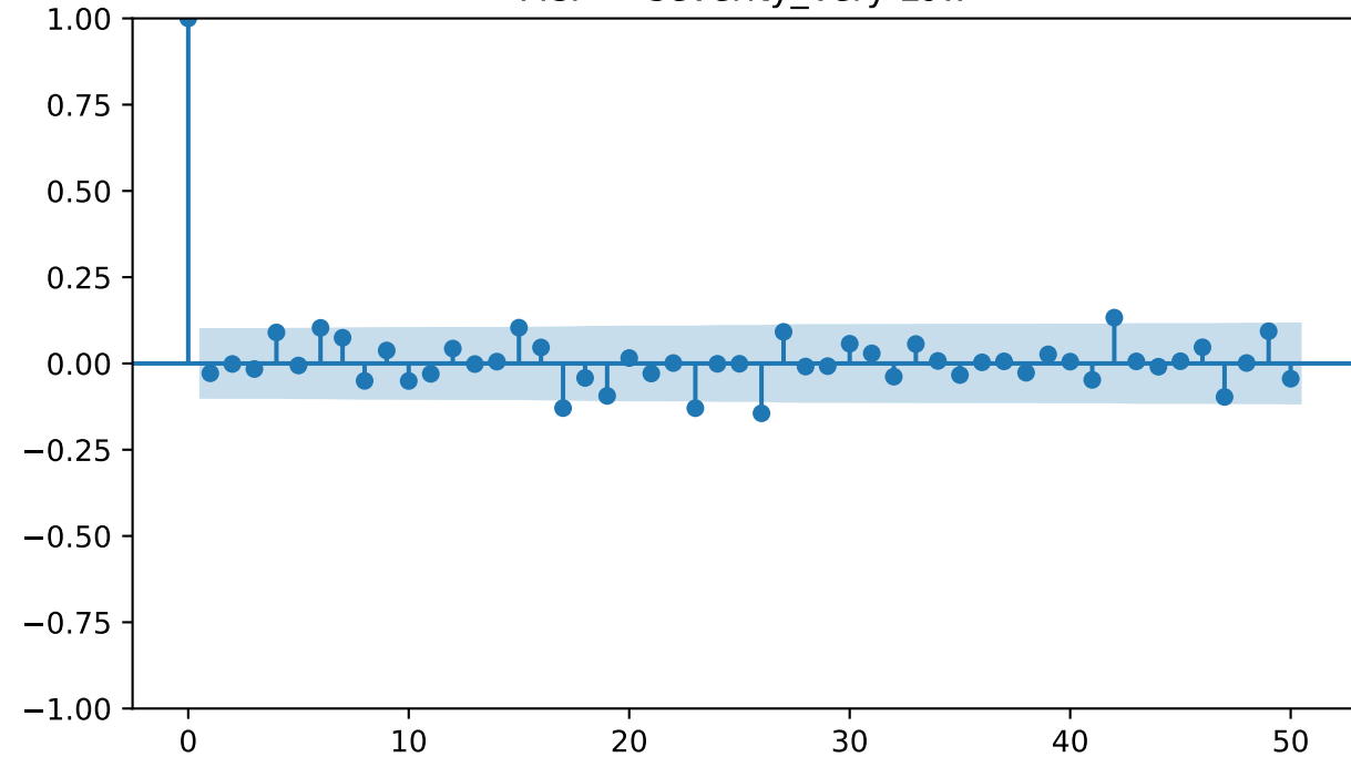
ACF — severity_Very Low
