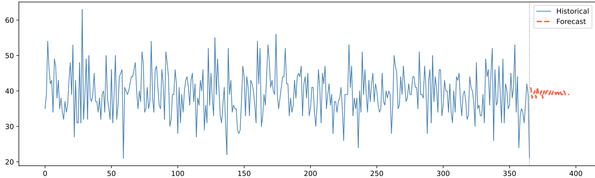
30-Day Forecast — severity_Medium
