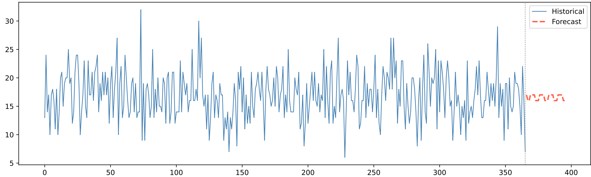
30-Day Forecast — severity_Very Low
