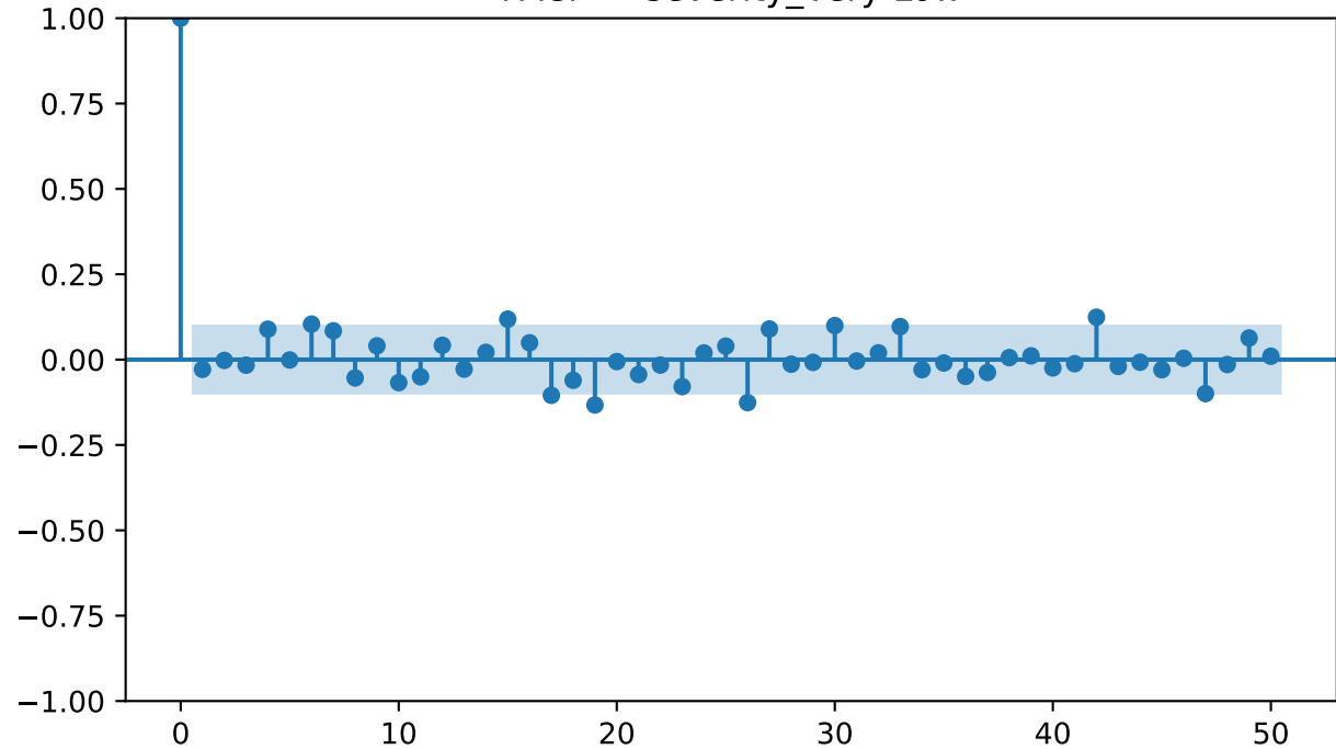
PACF — severity_Very Low
