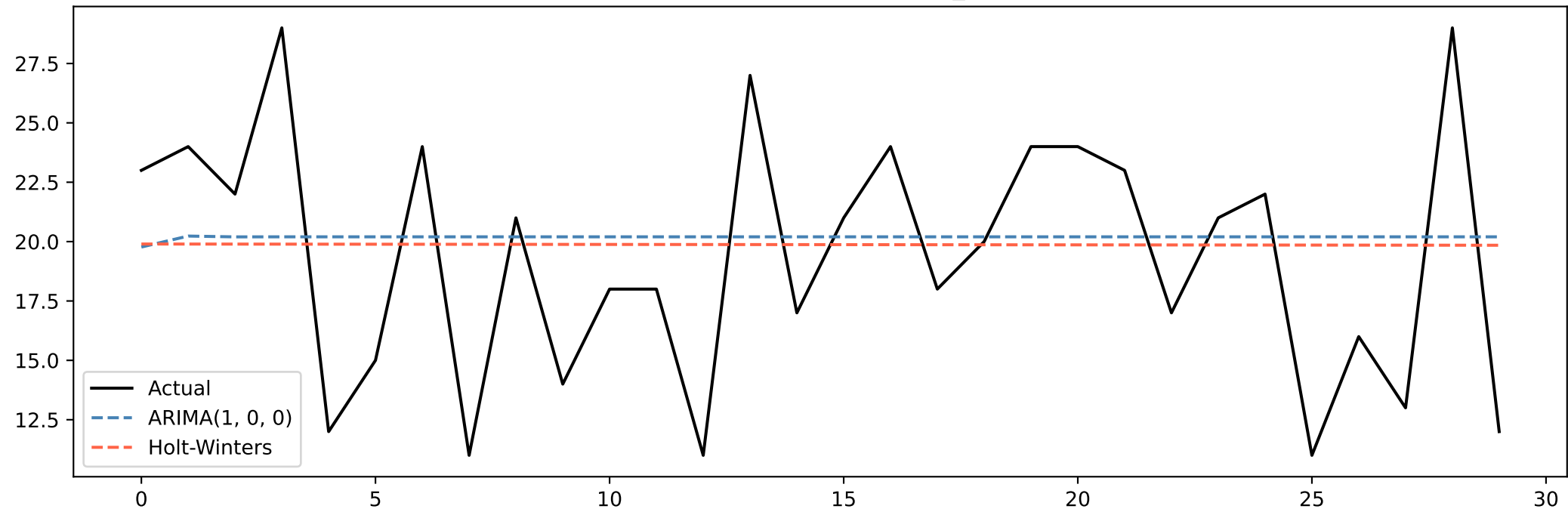
Model Comparison — severity_Critical
