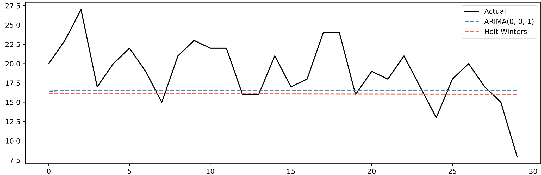
Model Comparison — severity_Low
