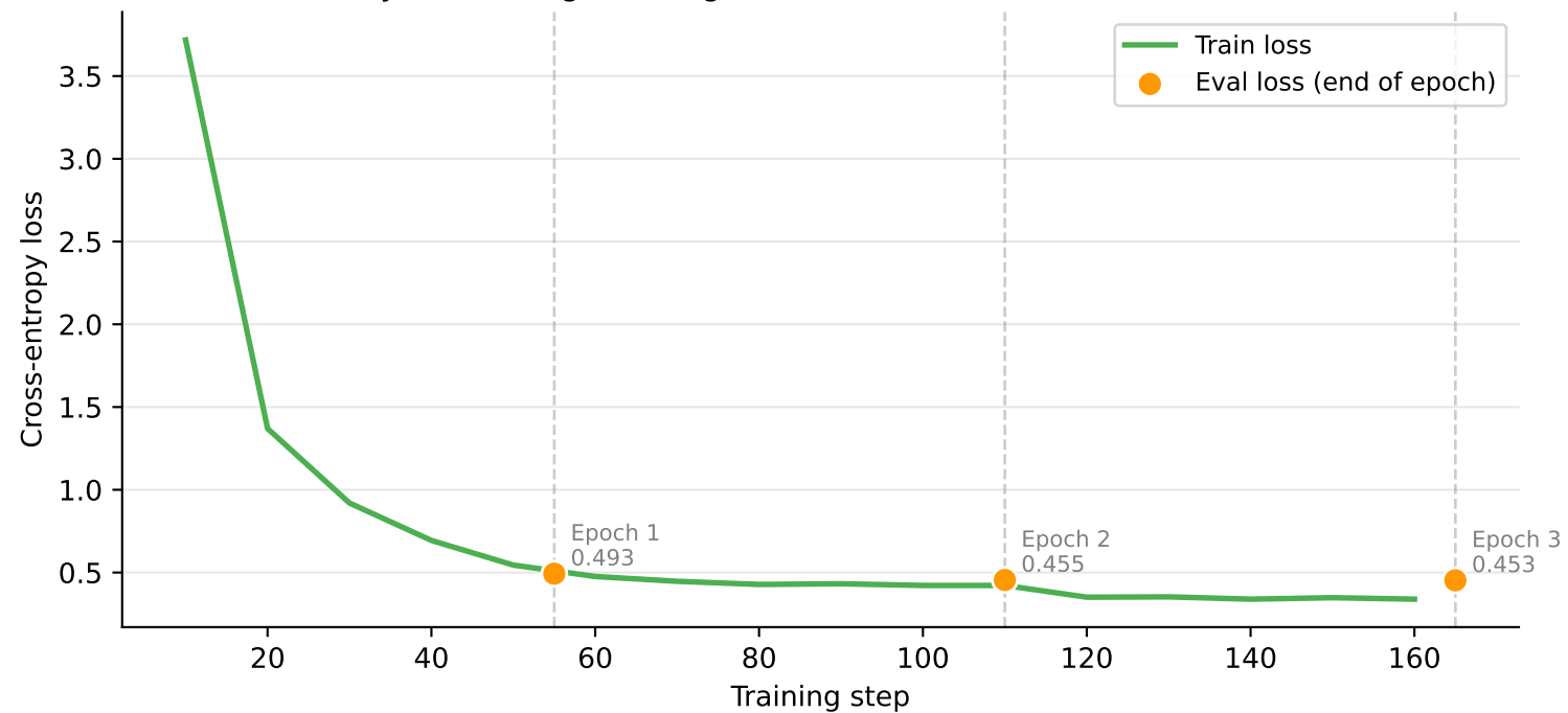
Safety Fine-tuning: Training Loss (AdvBench + HarmBench refusals)
