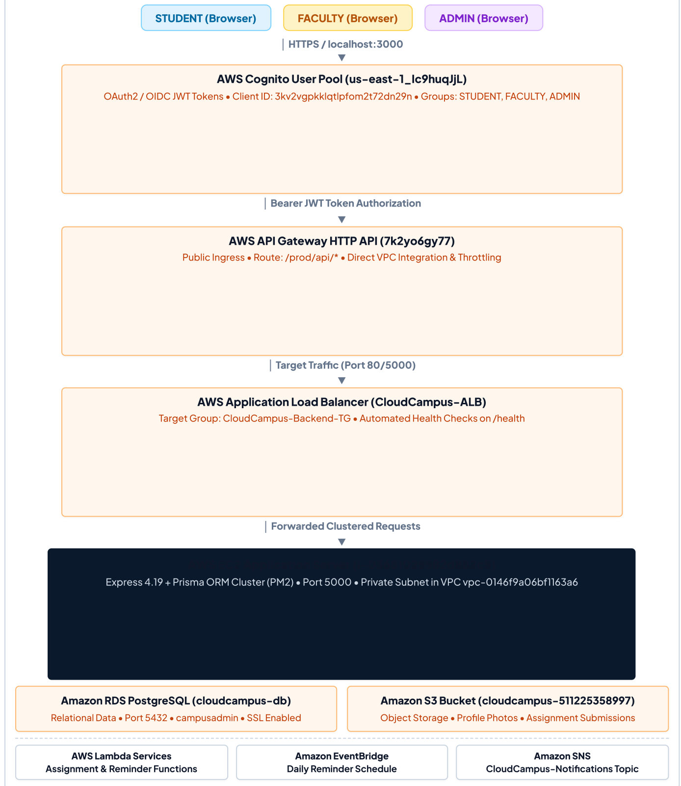
FIGURE 5.1 — FULL-PAGE MULTI-TIER CLOUD DEPLOYMENT ARCHITECTURE DIAGRAM
