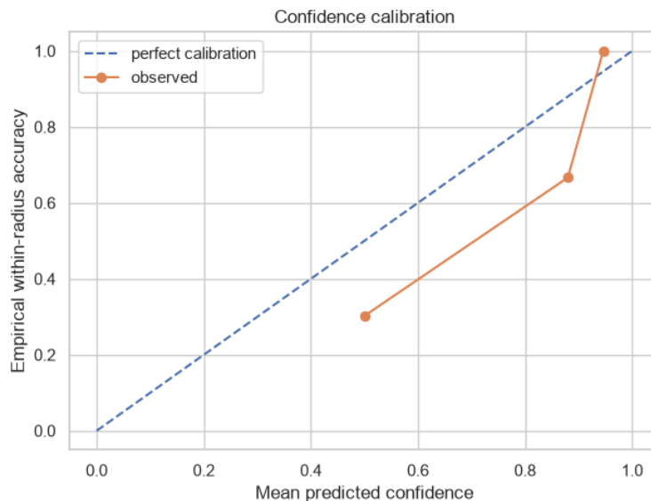
Figure 6. Confidence calibration: mean predicted confidence against empirical within-250 m accuracy, with the perfect-calibration diagonal.
