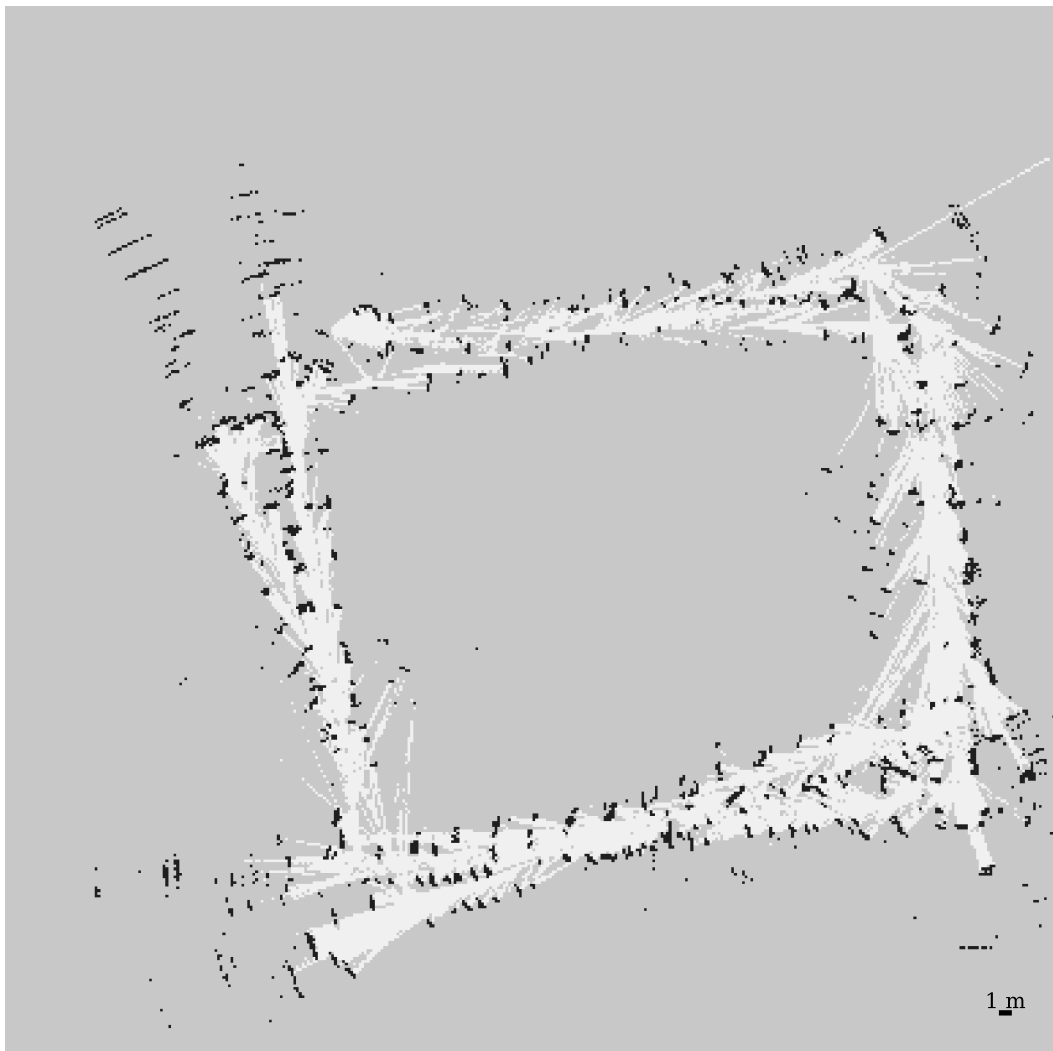
Experiment 3: Corridor Full-Run Occupancy Map
