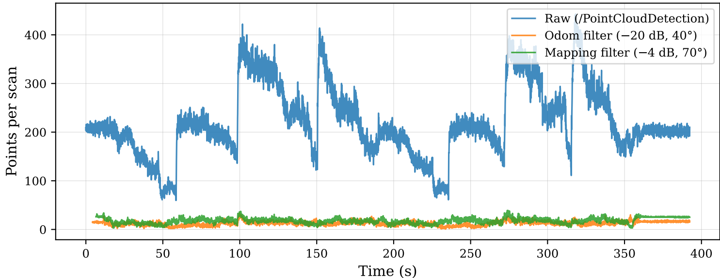
ARS548 Radar — Points per Scan After Each Preprocessing Filter
