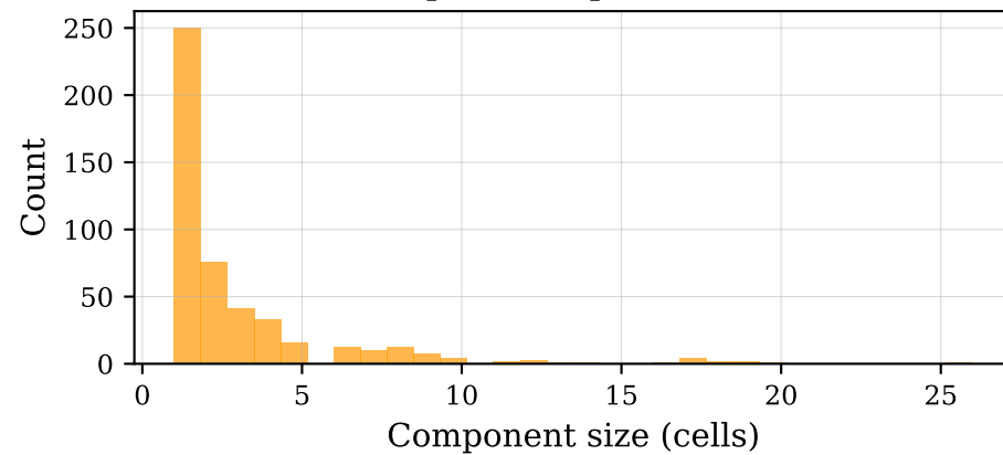
Occupied component sizes
