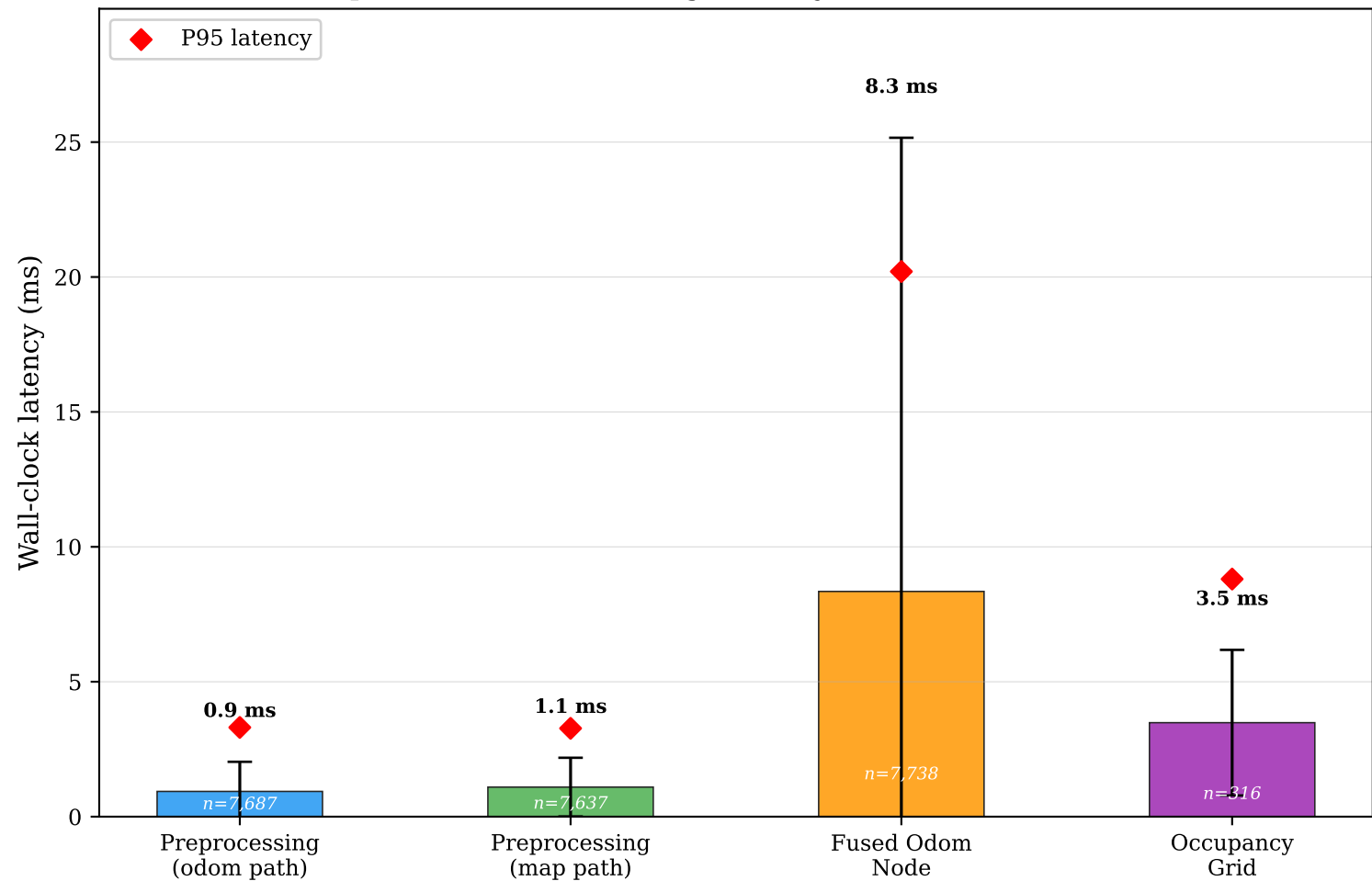
Pipeline Node Processing Latency (mean \pm std, \blacklozenge P95)
