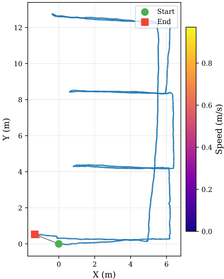
Fused Odometry Trajectory (total = 71.6 m, drift = 1.44 m = 2.0%)
