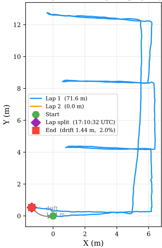
Two-Lap Trajectory — Drift = 1.44 m (2.0%) after 71.6 m total (Residual drift requires future pose-graph optimisation)
