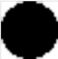
Near-full
