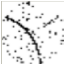
Scratch
