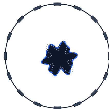
Deep Ensemble Mean ( K=5 ) IoU = 0.8926 | RMS = 376.9 mm
