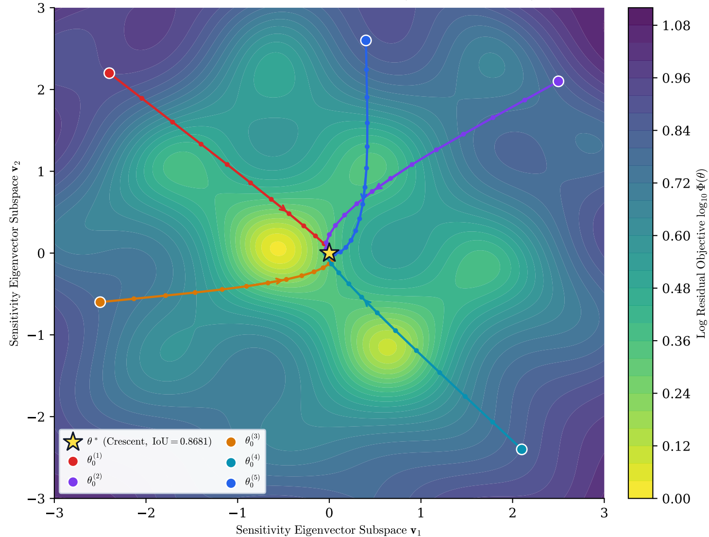
Multi-Start Levenberg--Marquardt Trajectories (Target #9: Crescent)
