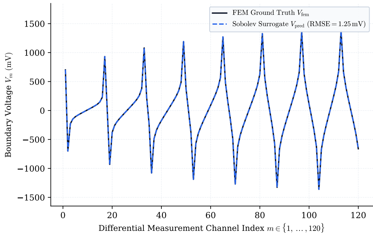
(b) Representative 120-Channel Differential Voltage Slice (Target #1: Circle)
