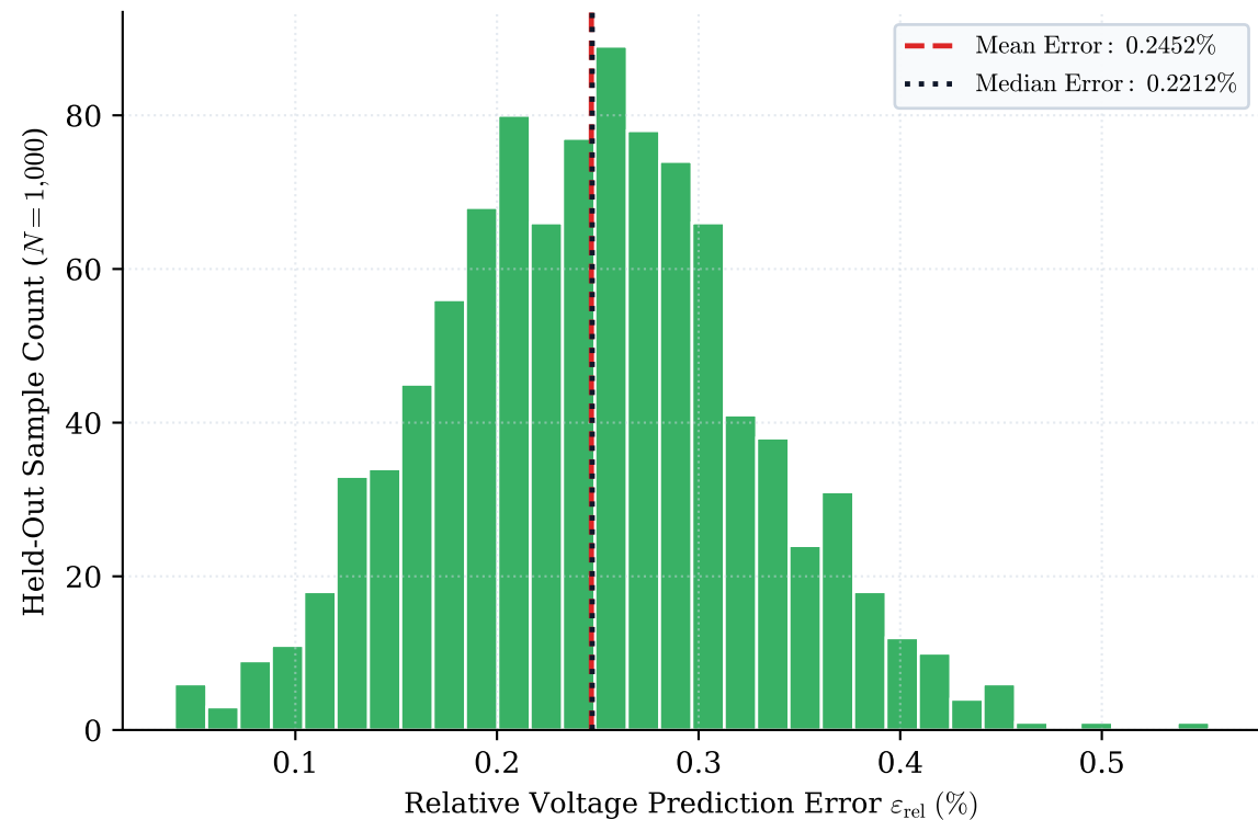
(a) Relative Voltage Error Distribution (1,000 Held-Out Samples)
