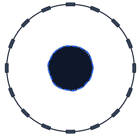
Deep Ensemble Mean ( K=5 ) IoU = 0.9379 | RMS = 628.7 mm
