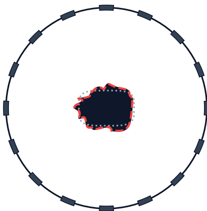
Deterministic Sobolev Surrogate IoU = 0.8500 | RMS = 124.8 mm
