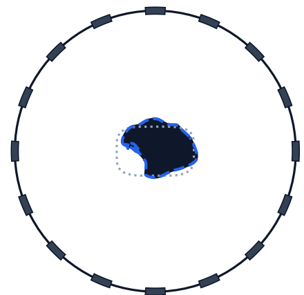
Deep Ensemble Mean ( K=5 ) IoU = 0.8500 | RMS = 159.9 mm
