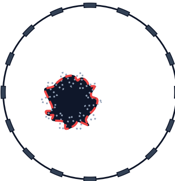
Deterministic Inversion IoU = 0.7749 | RMS = 33.2 mm
