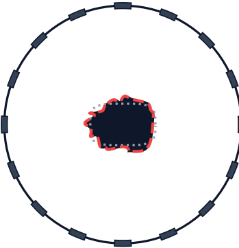
Deterministic Inversion IoU = 0.9039 | RMS = 17.1 mm
