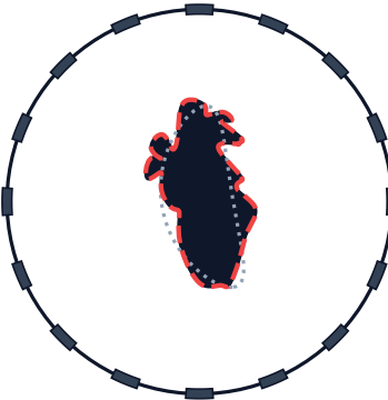
Deterministic Inversion IoU = 0.6401 | RMS = 45.2 mm
