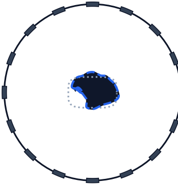
Ensemble Mean IoU = 0.9557 | RMS = 8.4 mm
