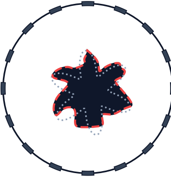
Deterministic Inversion IoU = 0.7317 | RMS = 43.2 mm
