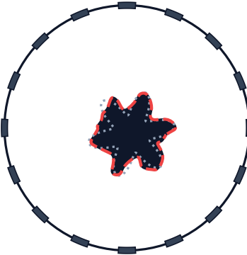
Deterministic Inversion IoU = 0.8681 | RMS = 35.7 mm
