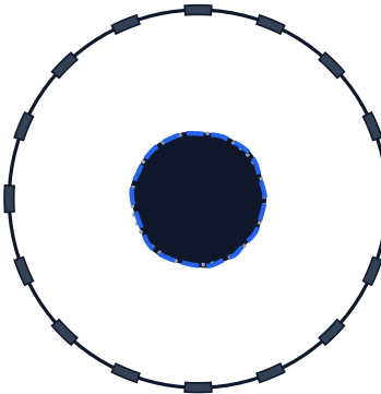
Ensemble Mean IoU = 0.9377 | RMS = 12.5 mm
