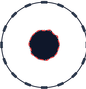
Deterministic Inversion IoU = 0.9034 | RMS = 18.7 mm
