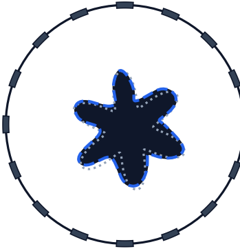
Ensemble Mean IoU = 0.7405 | RMS = 41.6 mm
