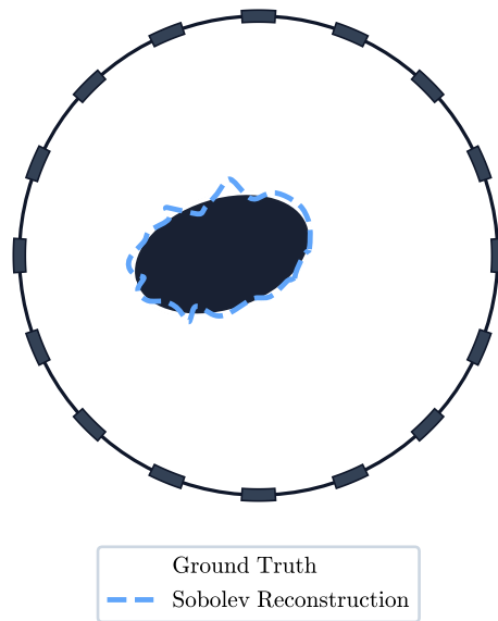
(b) Sobolev Surrogate (IoU = 0.9034)
