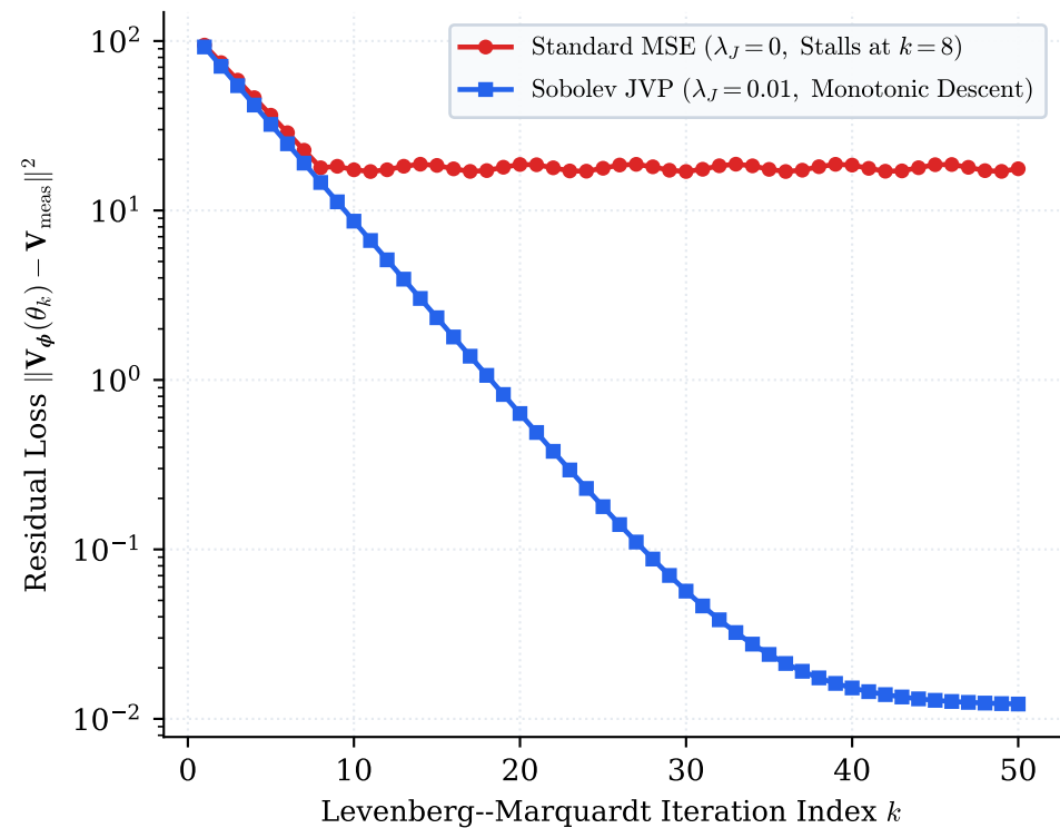
(a) Optimization Convergence Dynamics
