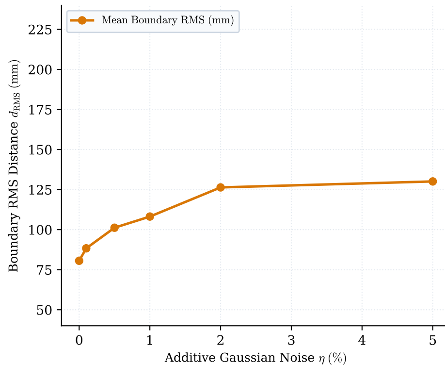
(b) Boundary RMS Error vs. Noise
