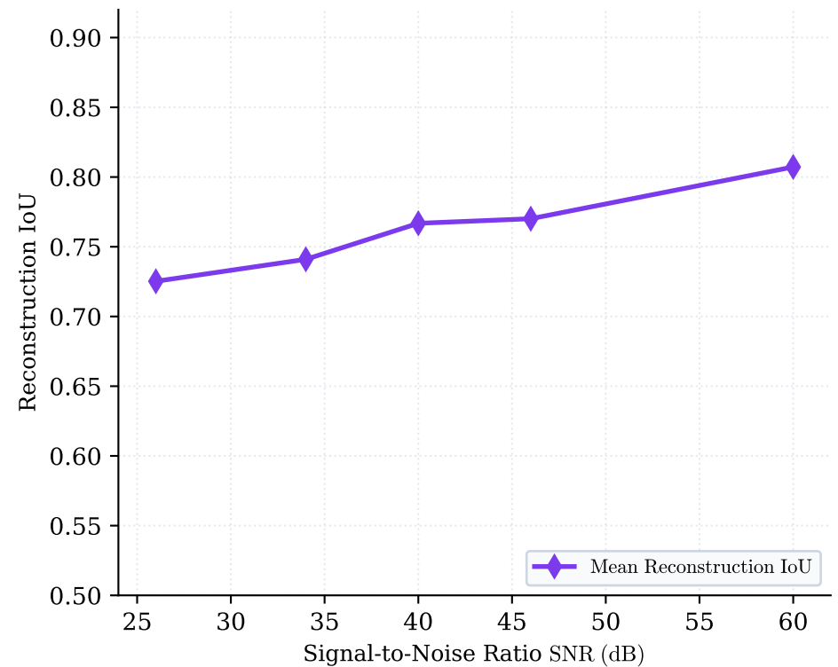
(c) Reconstruction Accuracy vs. SNR
