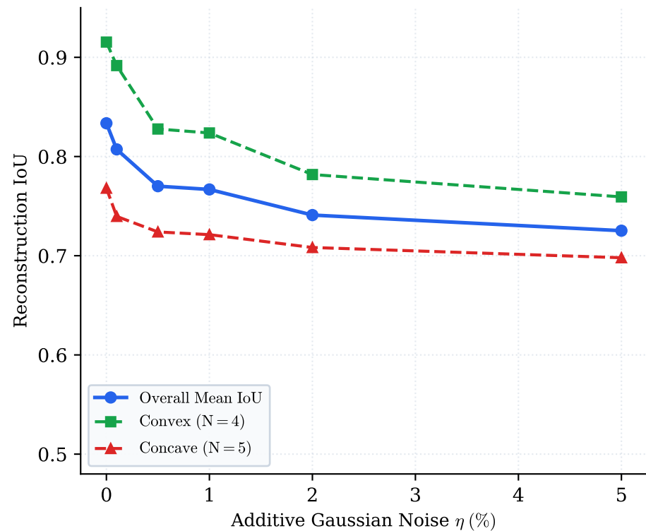
(a) Reconstruction Accuracy vs. Noise
