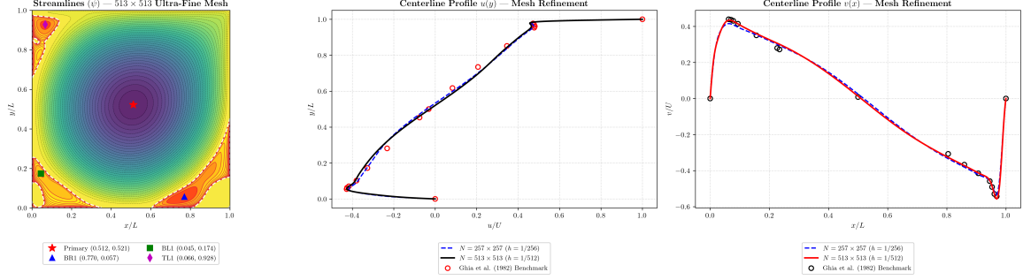
Figure 2: Grid refinement comparison at Re = 10,000 : 257 \times 257 (66,049 nodes) vs. 513 \times 513 (263,169 nodes), demonstrating asymptotic convergence of centerline velocity profiles and resolving thin wall boundary layers.
