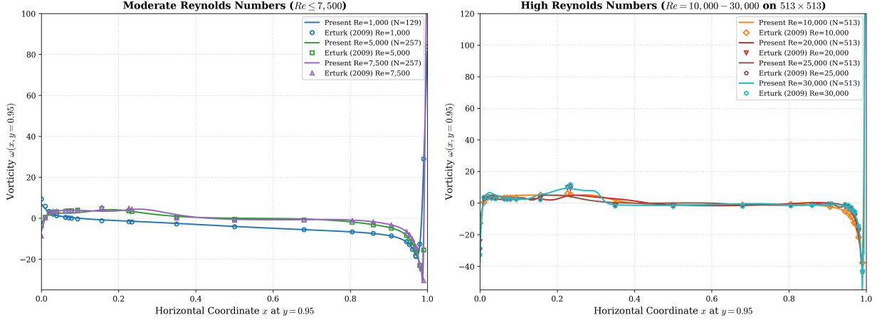
Figure 3: Benchmark validation against Erturk (2009) [11] (Table 3): Vorticity \omega(x, y = 0.95) along the near-lid horizontal cut for moderate ( Re \leq 7,500 ) and high ( Re = 10,000 - 30,000 on 513 \times 513 ) Reynolds numbers. Solid lines represent present solver results; discrete markers denote benchmark data.
