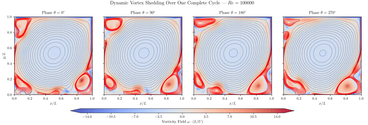
(c) Instantaneous 4-Phase Vorticity and Streamline Fields Over Shedding Cycle
