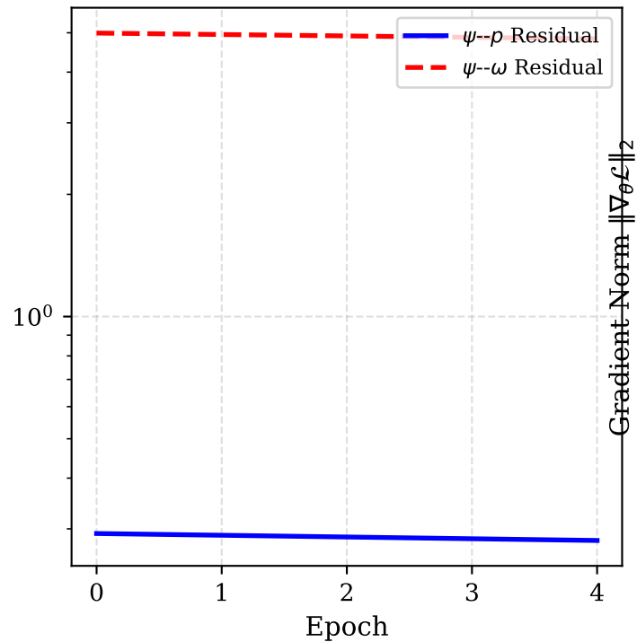
PDE Residual Evolution
