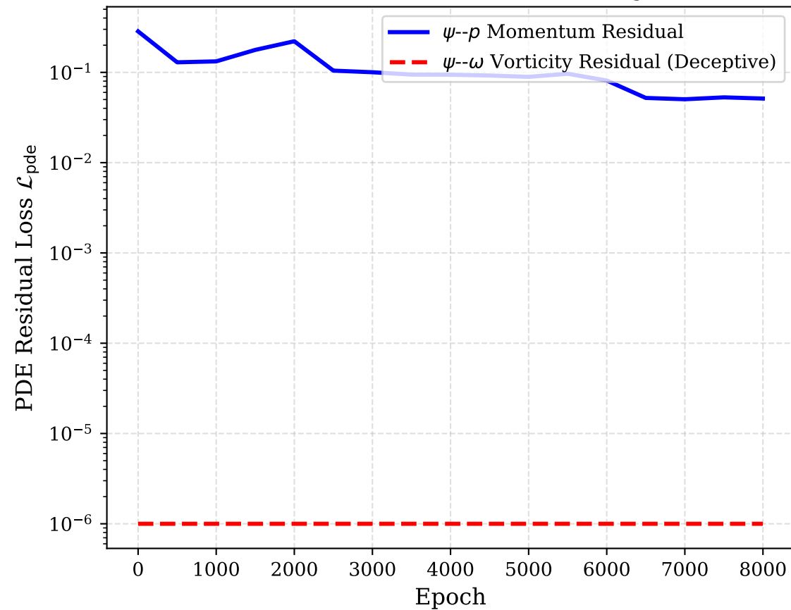
PDE Residual Evolution (False Convergence)
