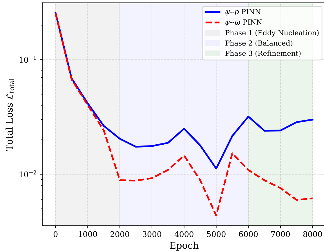
Total Training Loss Trajectory
