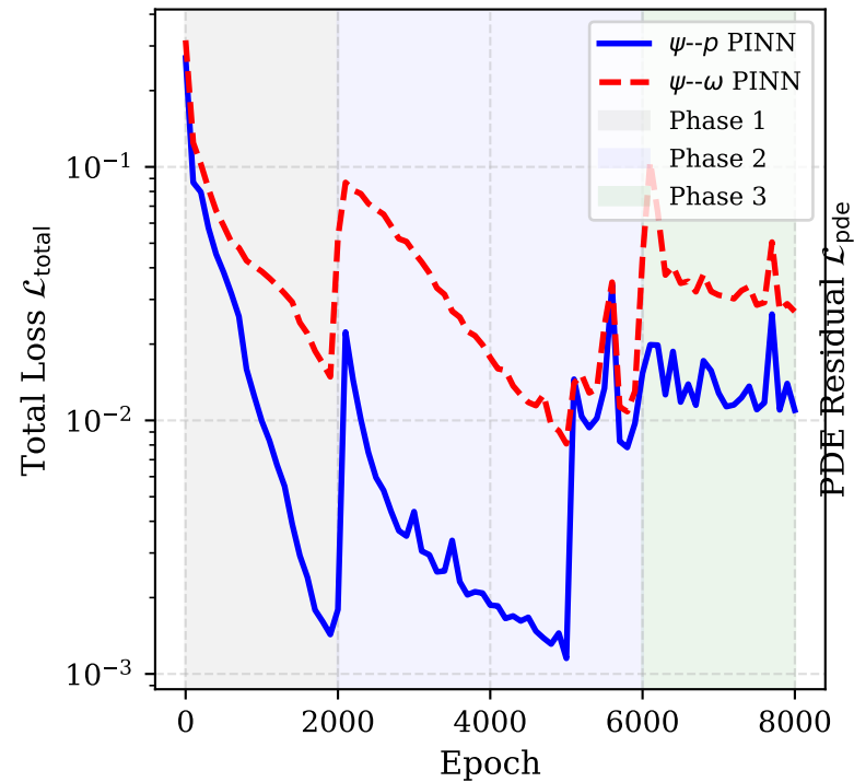
Total Training Loss
