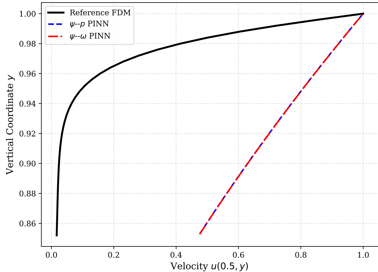
Top Boundary-Layer Shear Zoom ( y > 0.85 )
