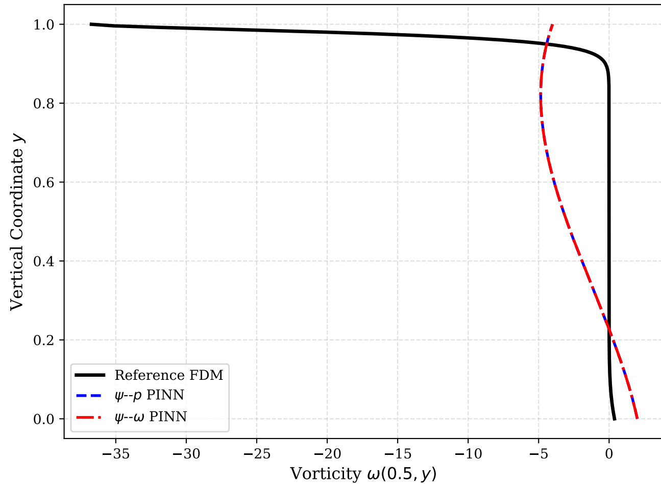
Centerline Vorticity Distribution
