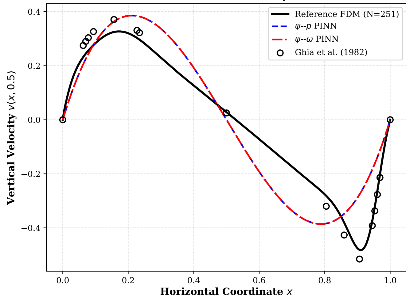
Horizontal Centerline Velocity Profile
