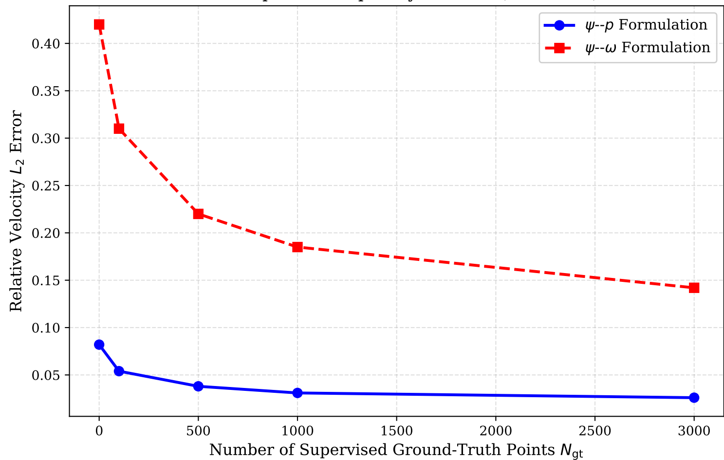
Data Supervision Sparsity Ablation (Re = 1000)
