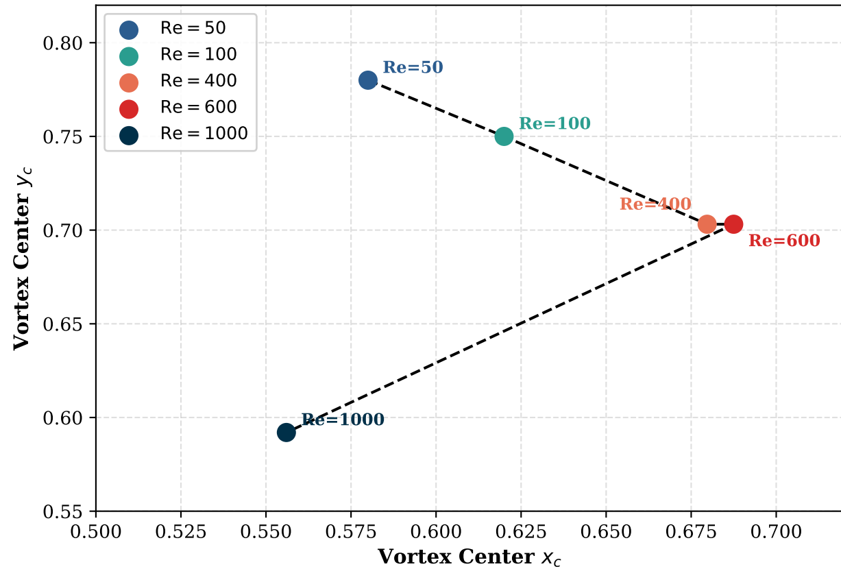
(c) Primary Vortex Core Migration Trajectory
