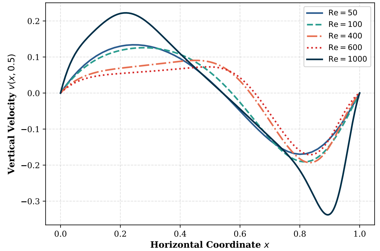
(b) Horizontal Centerline Velocity v(x, 0.5) vs Re
