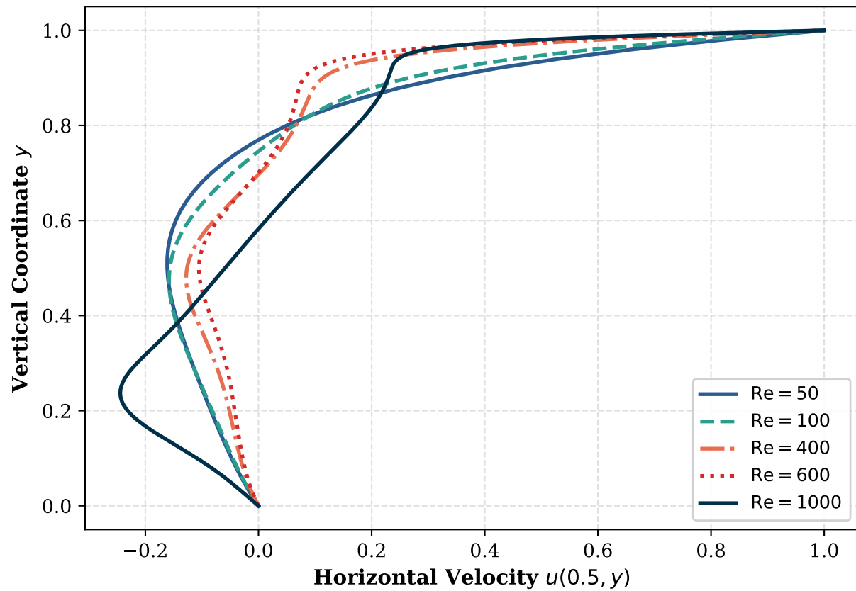
(a) Vertical Centerline Velocity u(0.5, y) vs Re
