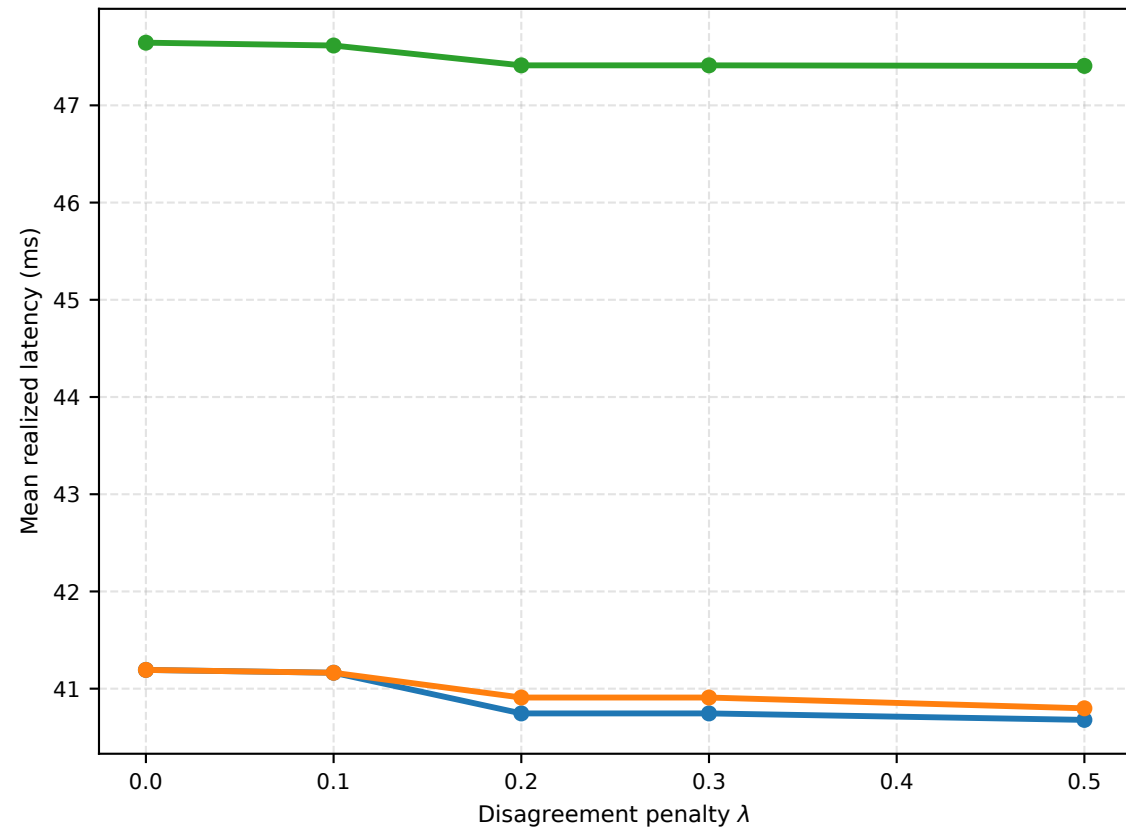
Consensus Penalty Sweep: Latency
