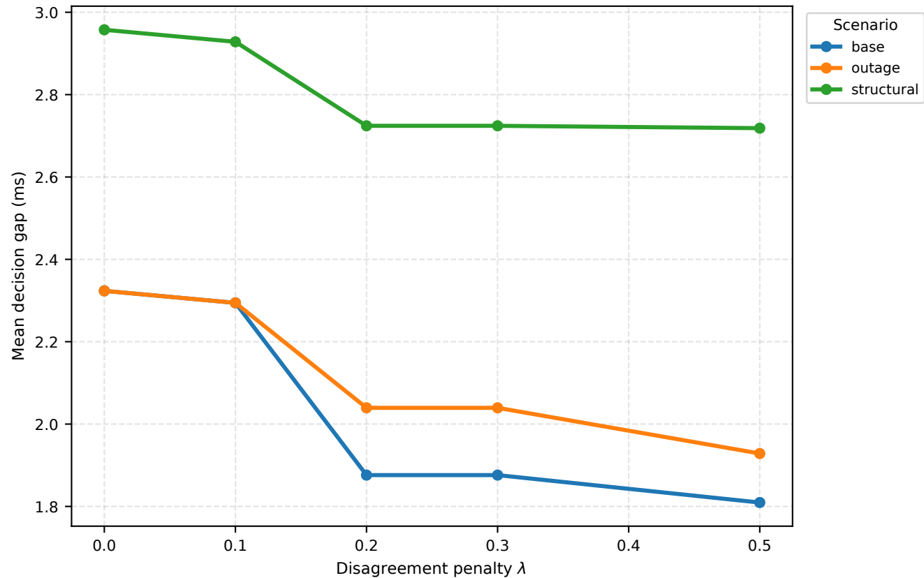
Consensus Penalty Sweep: Decision Gap
