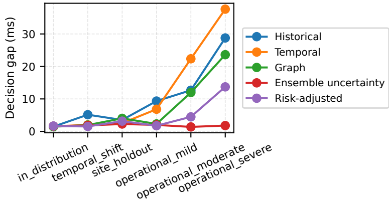
Decision Gap Under Shift
