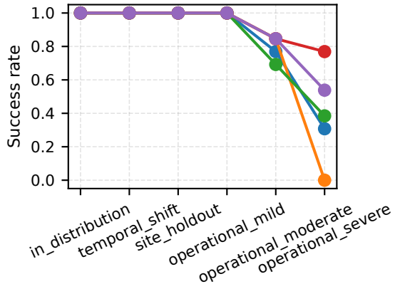
QoS Success Under Shift
