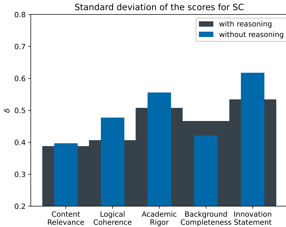
Figure 4.5.: Comparison of the standard deviation of the computed ranking scores for each evaluation dimension when the judge is instructed with versus without asking to provide reasoning.
