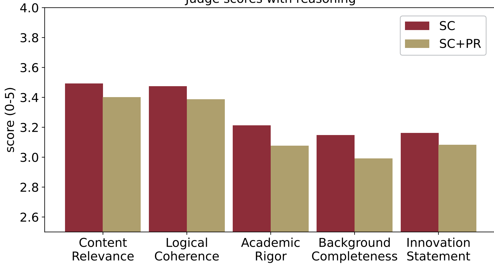
Judge scores with reasoning
