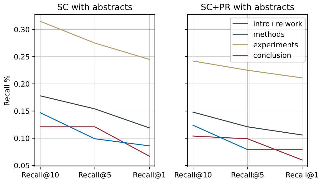
Figure 4.2.: Comparison of single-step retrieval performance between ScholarCopilot (SC) with and without passage retrieval (PR) on context with abstracts (this resembles generated context more closely).
