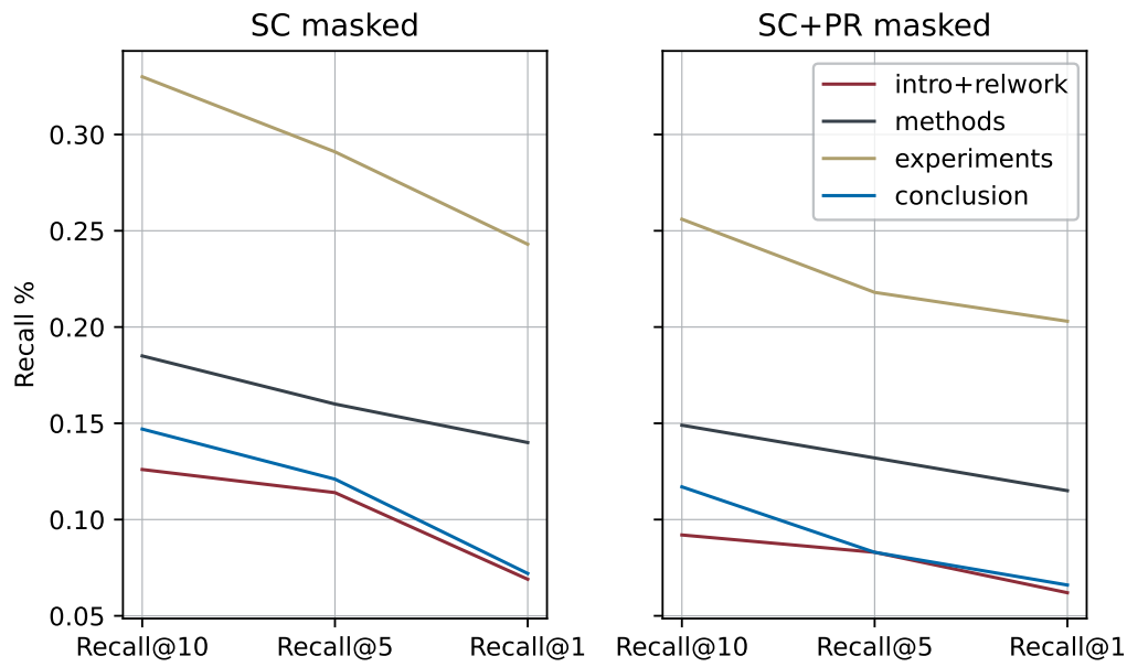
Figure 4.1.: Comparison of single-step retrieval performance between ScholarCopilot (SC) with and without passage retrieval (PR) on context with masked citations. intro+relwork denotes context drawn from Introduction and Related Work sections.
