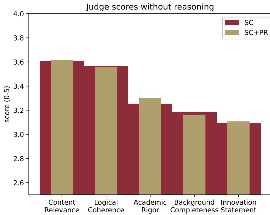
Figure 4.4.: Comparison of the generation quality scores between ScholarCopilot (SC) with and without passage retrieval (PR) when the judge is instructed to only provide scores.
