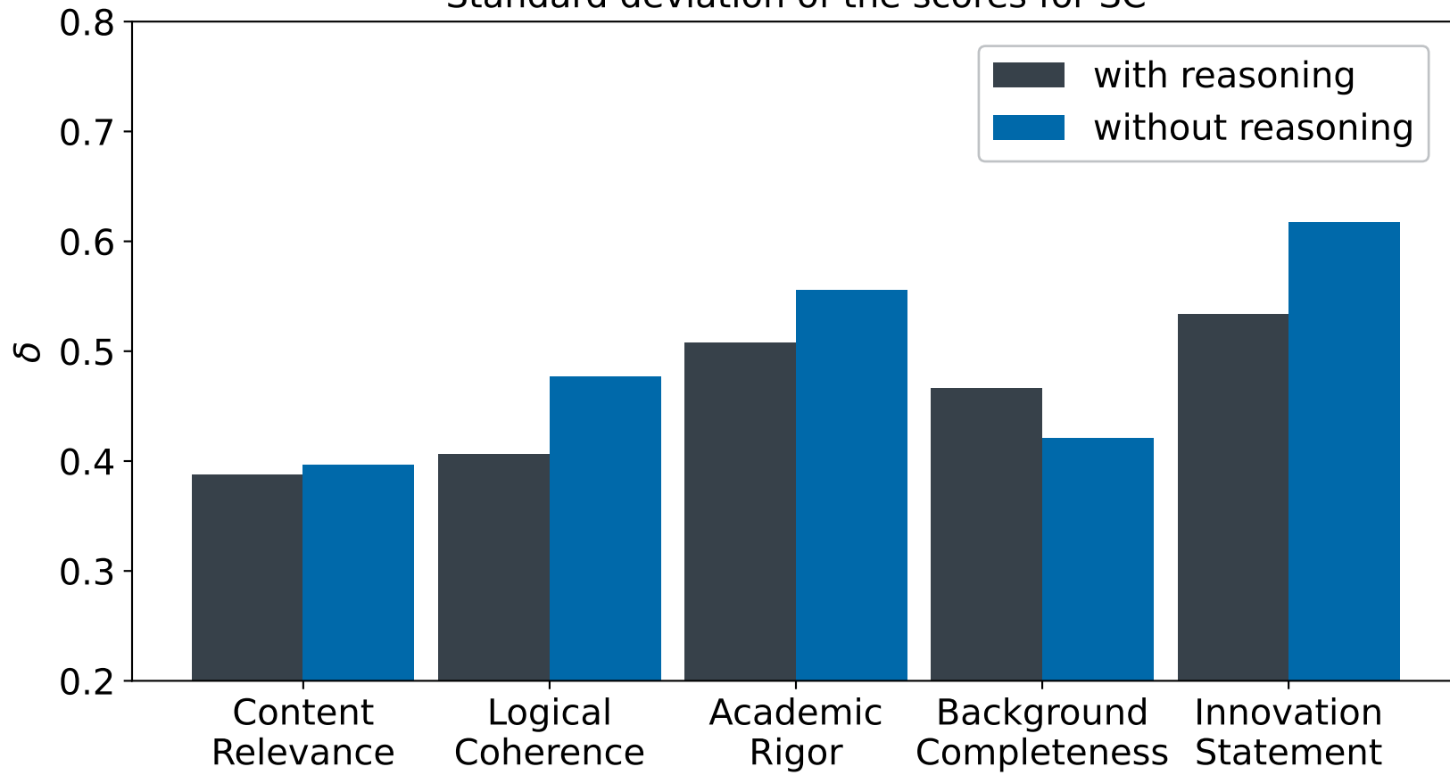
Standard deviation of the scores for SC
