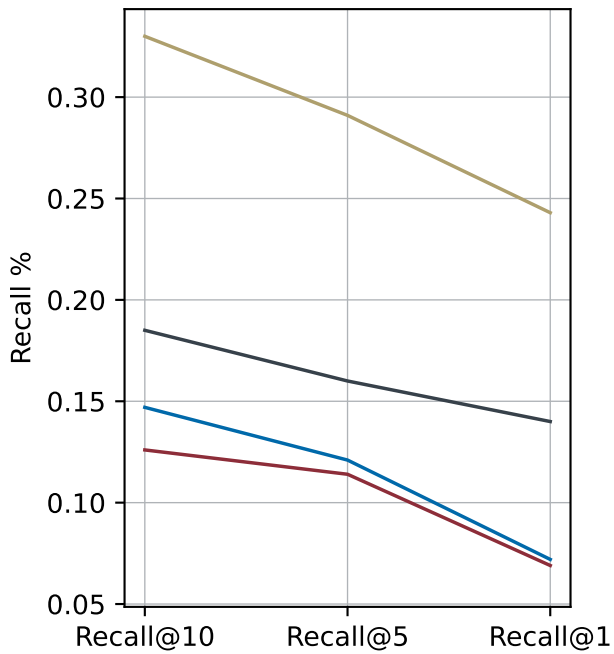
SC masked
