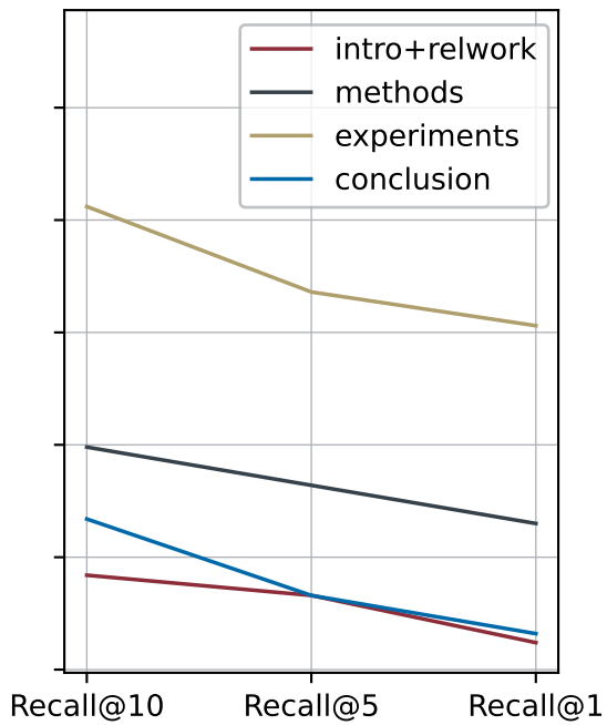
SC+PR masked
