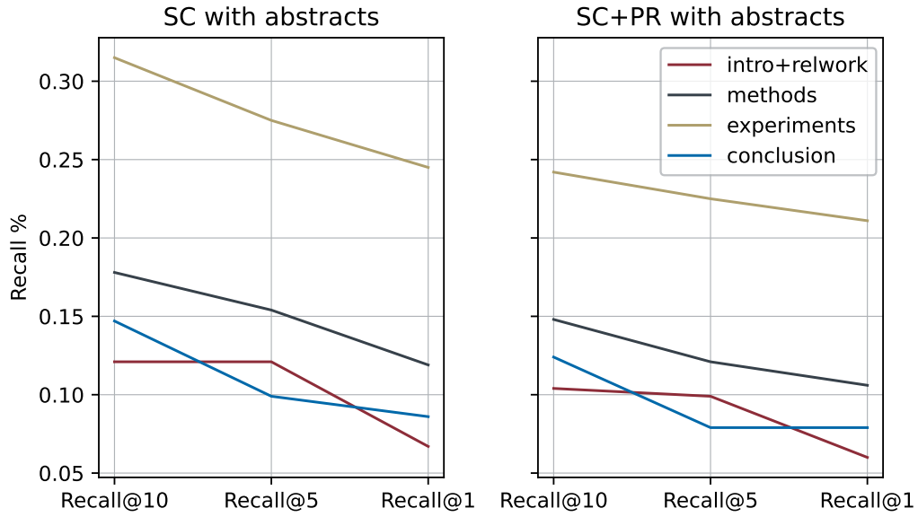
Figure 4.2.: Comparison of single-step retrieval performance between ScholarCopilot (SC) with and without passage retrieval (PR) on the with-abstracts dataset.
