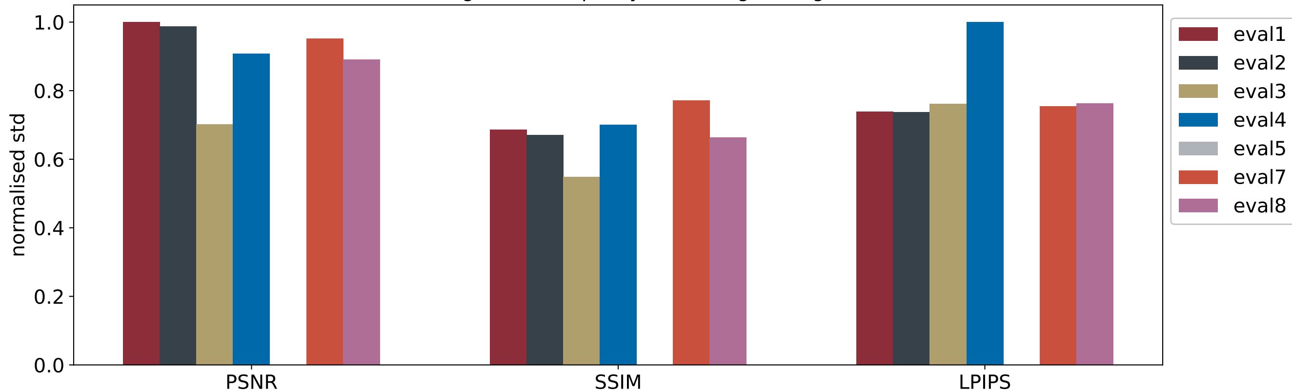
Std. of generation quality scores (right image)
