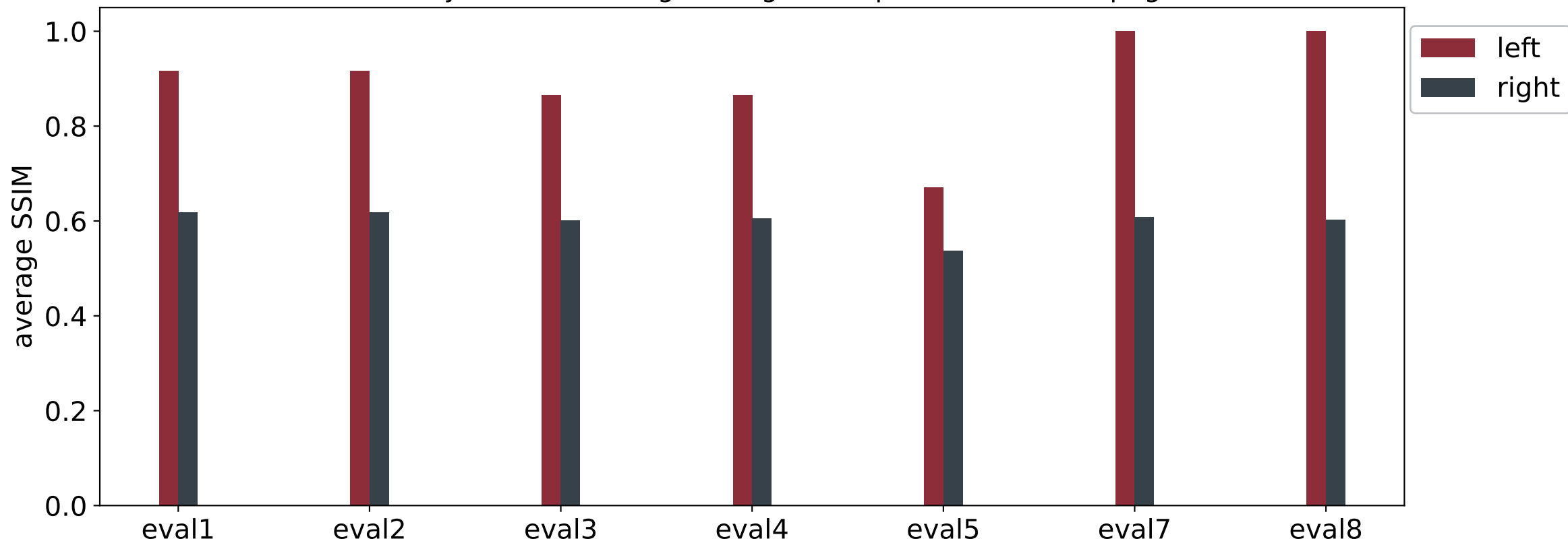
Structural Similarity Index of left/right images compared to their resp. ground truth
