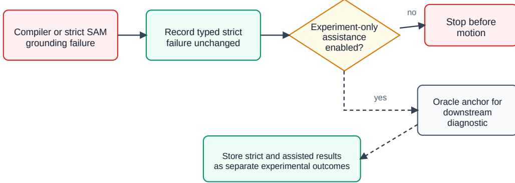
Figure 16: Experiment-only grounding-assistance subgraph. The strict failure remains recorded even when an oracle anchor permits a separate downstream diagnostic continuation.
