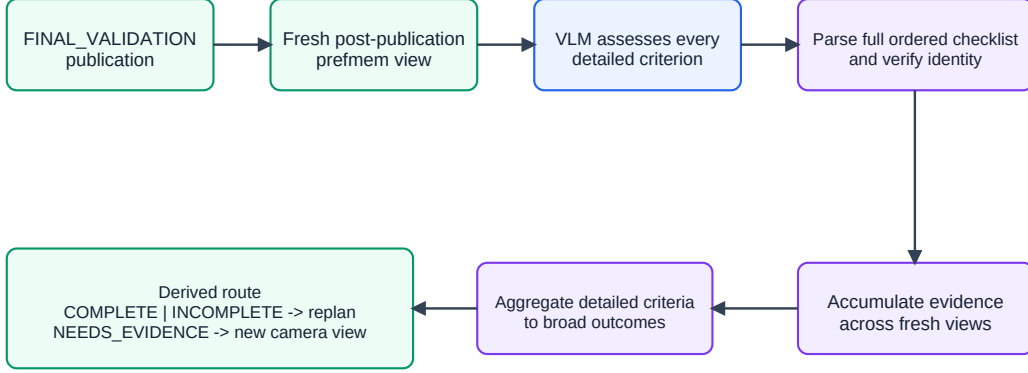
Figure 14: Validator final-assessment subgraph. Host code verifies the full ordered checklist, accumulates evidence across fresh views, and derives the final route from the frozen broad outcomes.
