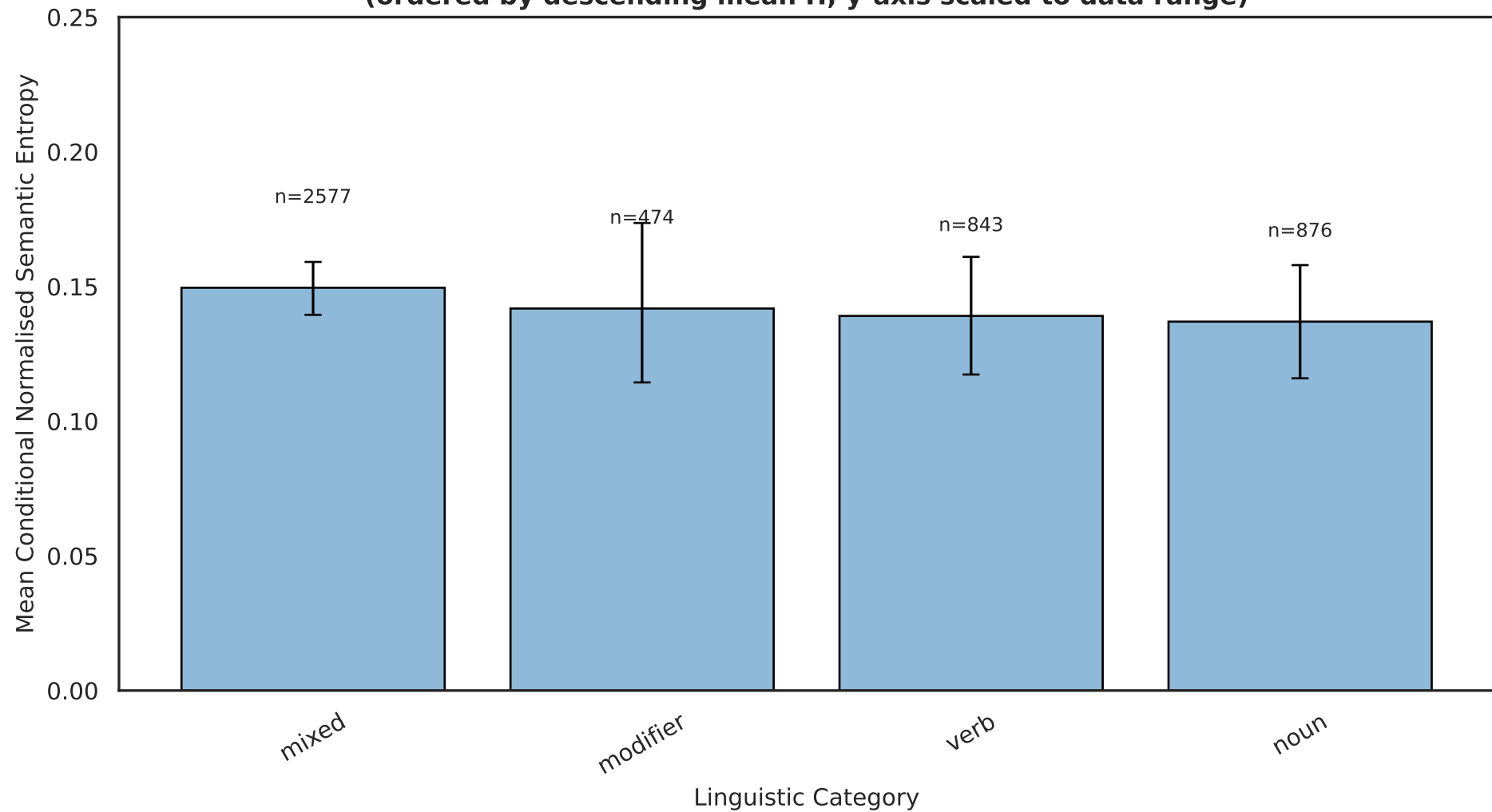
RQ1 Figure 2. Mean Semantic Entropy by Linguistic Category (ordered by descending mean \hat{H} ; y-axis scaled to data range)
