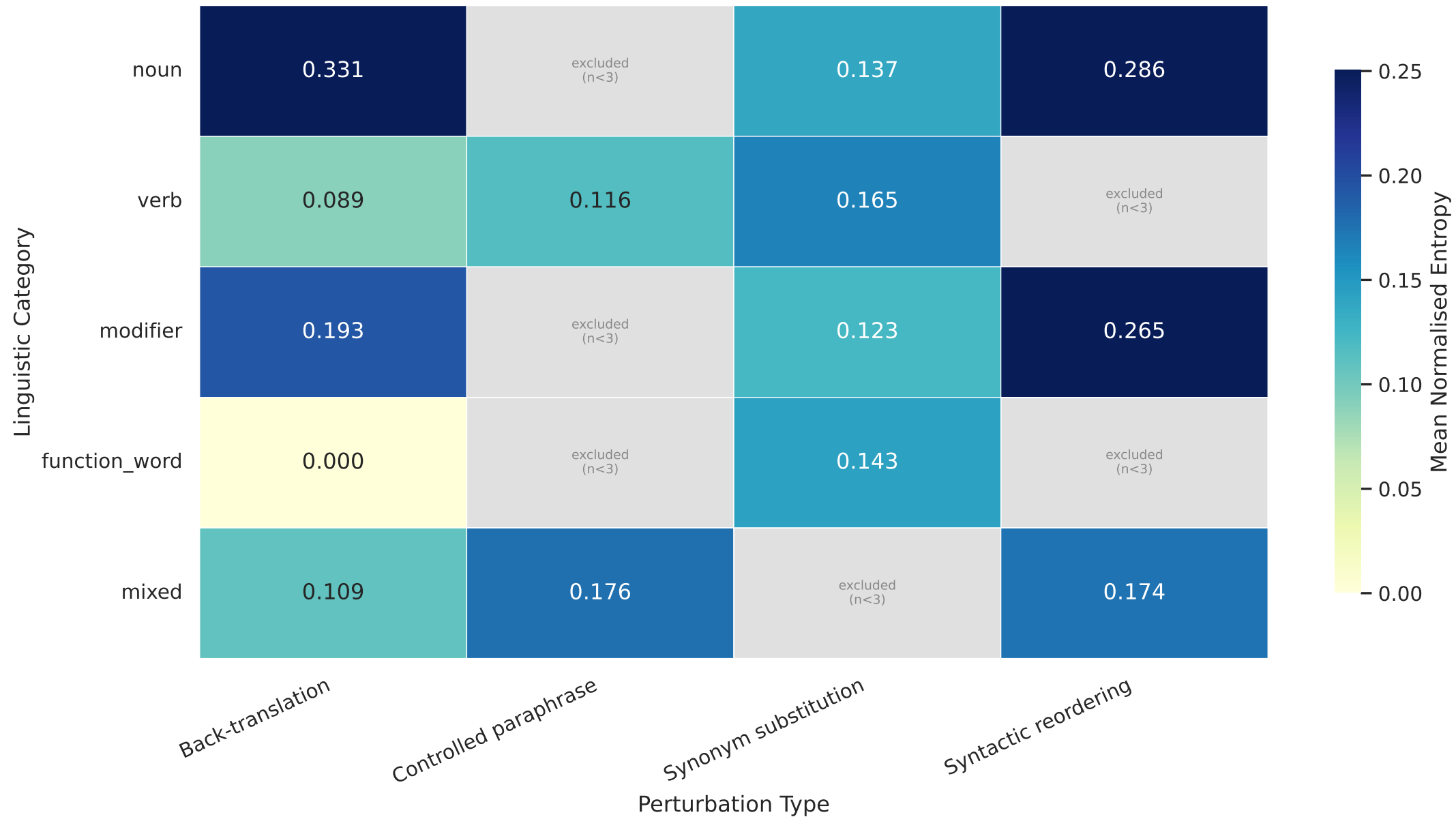
BERT-base | General domain - 110M parameters Figure E. Mean Entropy Heatmap (Type x Category)
