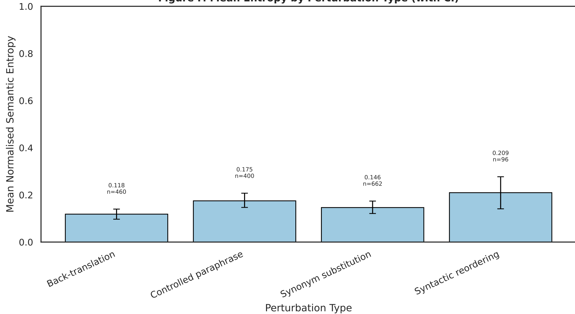
BERT-base | General domain - 110M parameters Figure F. Mean Entropy by Perturbation Type (with CI)
