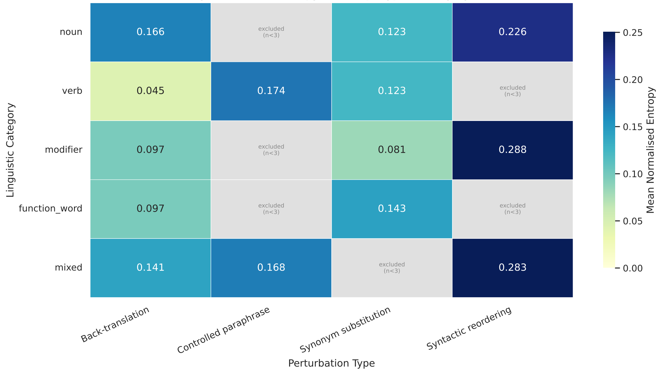
BioBERT | Biomedical domain - 110M parameters Figure E. Mean Entropy Heatmap (Type x Category)
