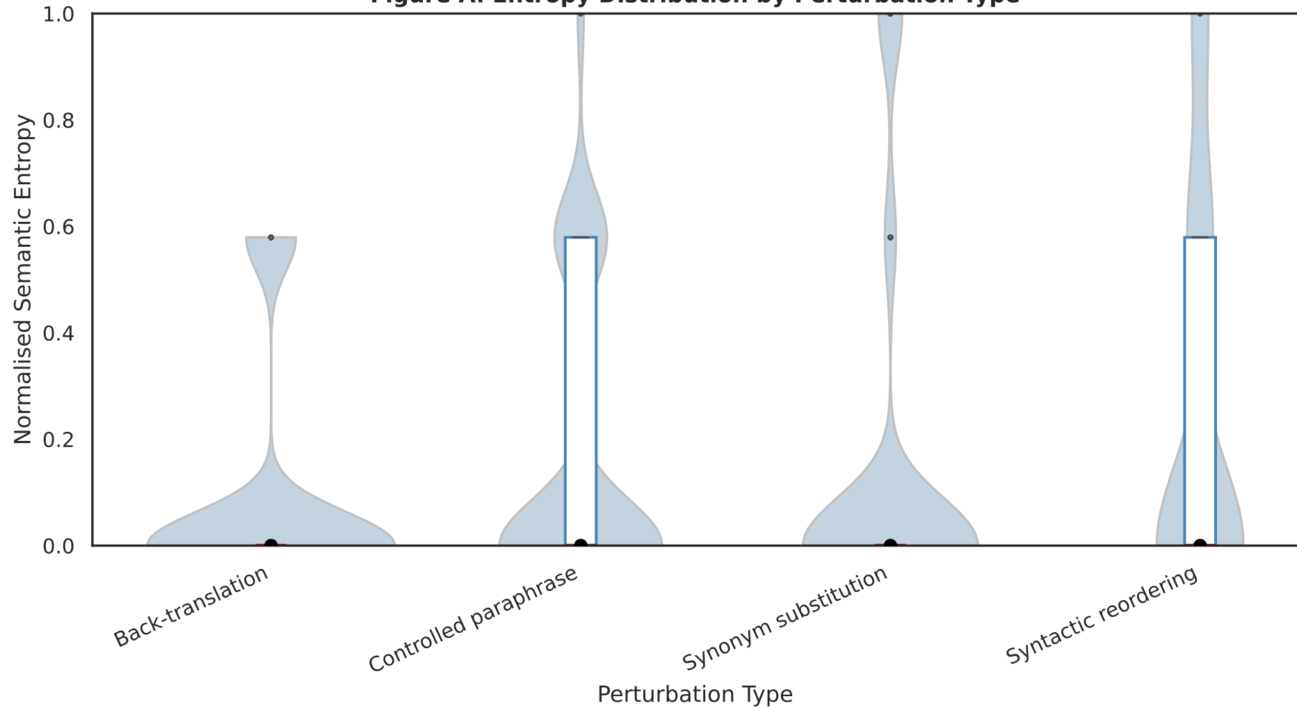
Figure A. Entropy Distribution by Perturbation Type
