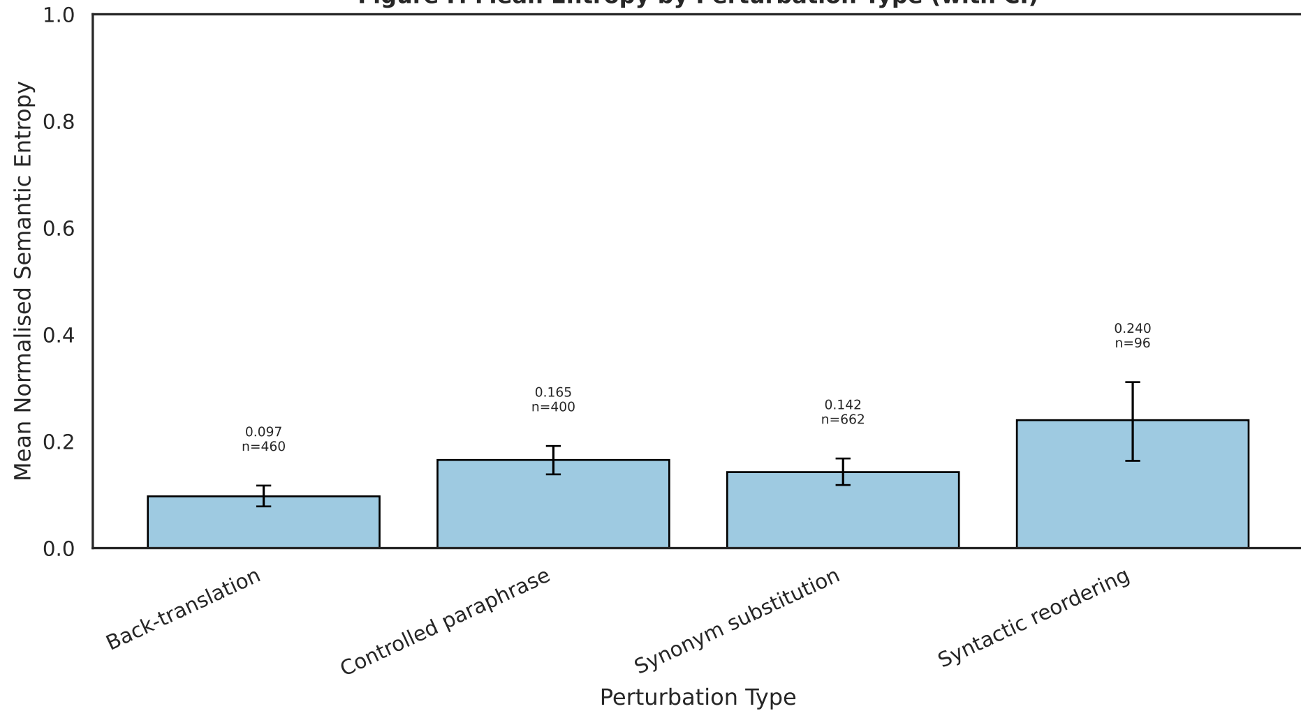
Figure F. Mean Entropy by Perturbation Type (with CI)
