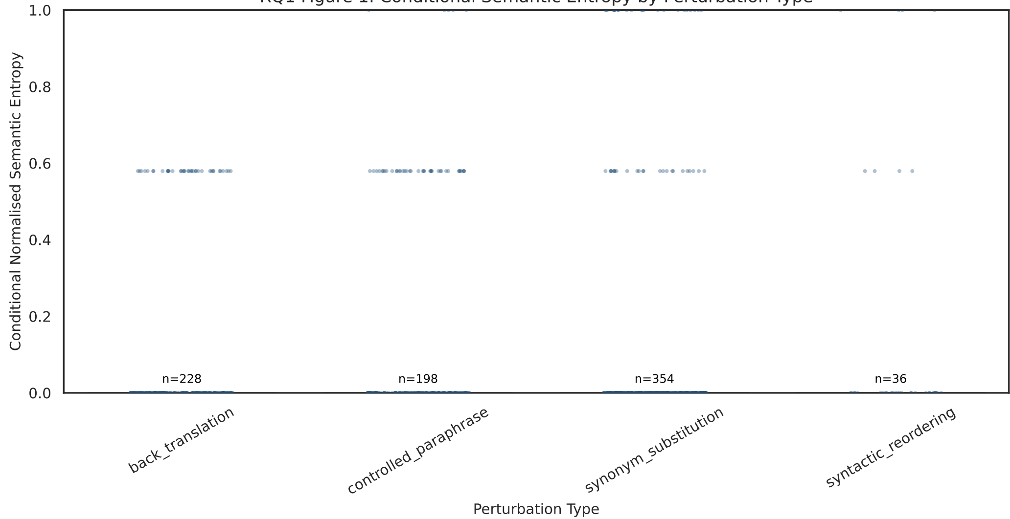
RQ1 Figure 1. Conditional Semantic Entropy by Perturbation Type
