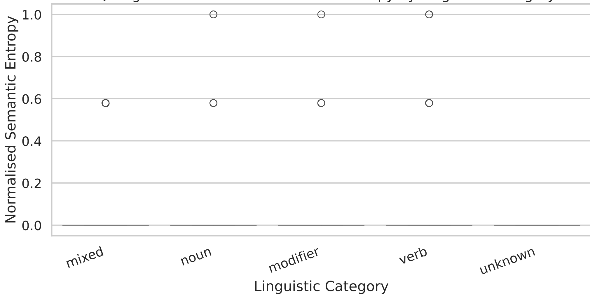
RQ1 Figure 2: Normalised Semantic Entropy by Linguistic Category
