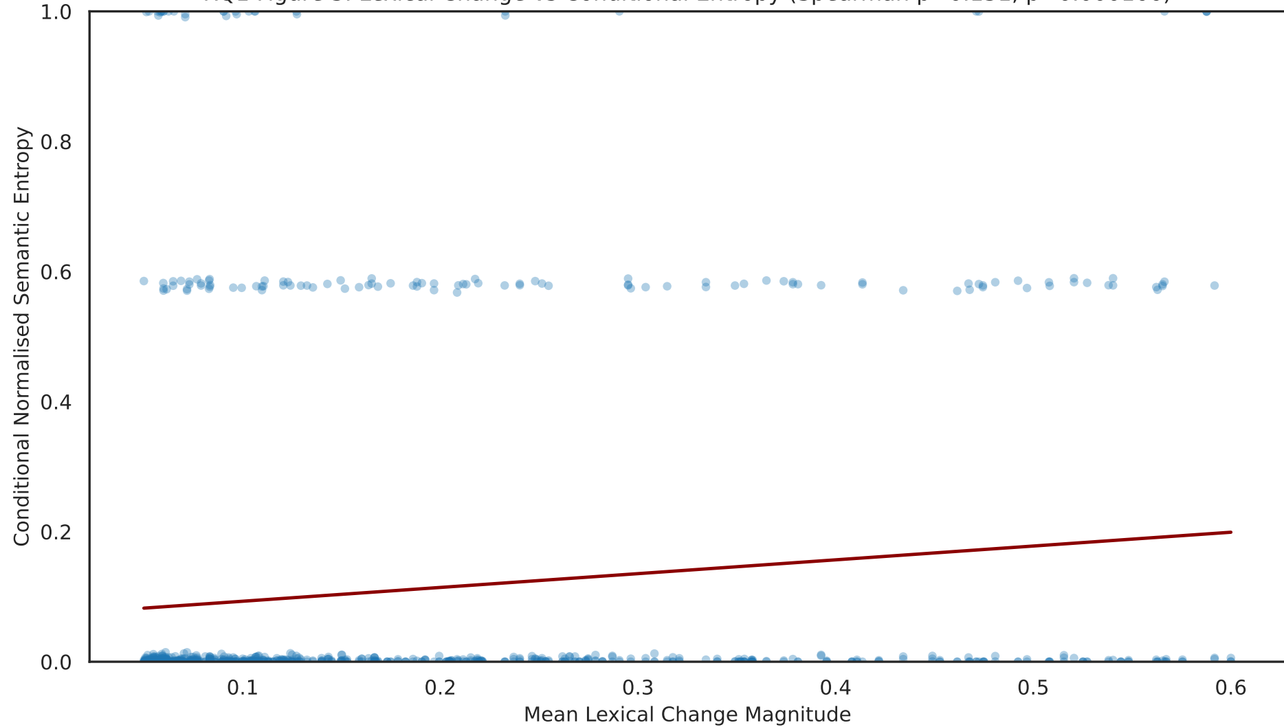
RQ1 Figure 3. Lexical Change vs Conditional Entropy (Spearman \rho=0.131 , p=0.000166 )
