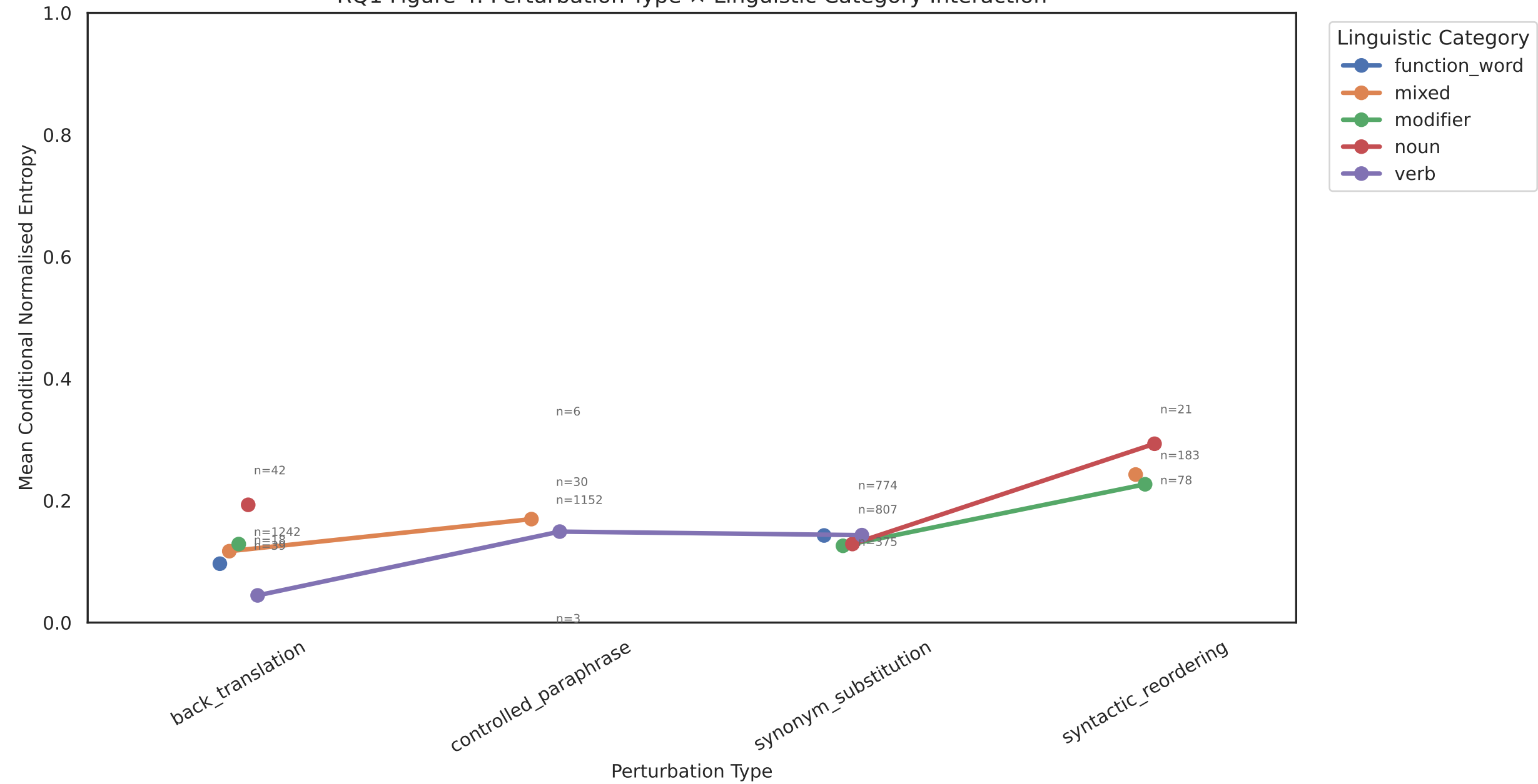
RQ1 Figure 4. Perturbation Type × Linguistic Category Interaction
